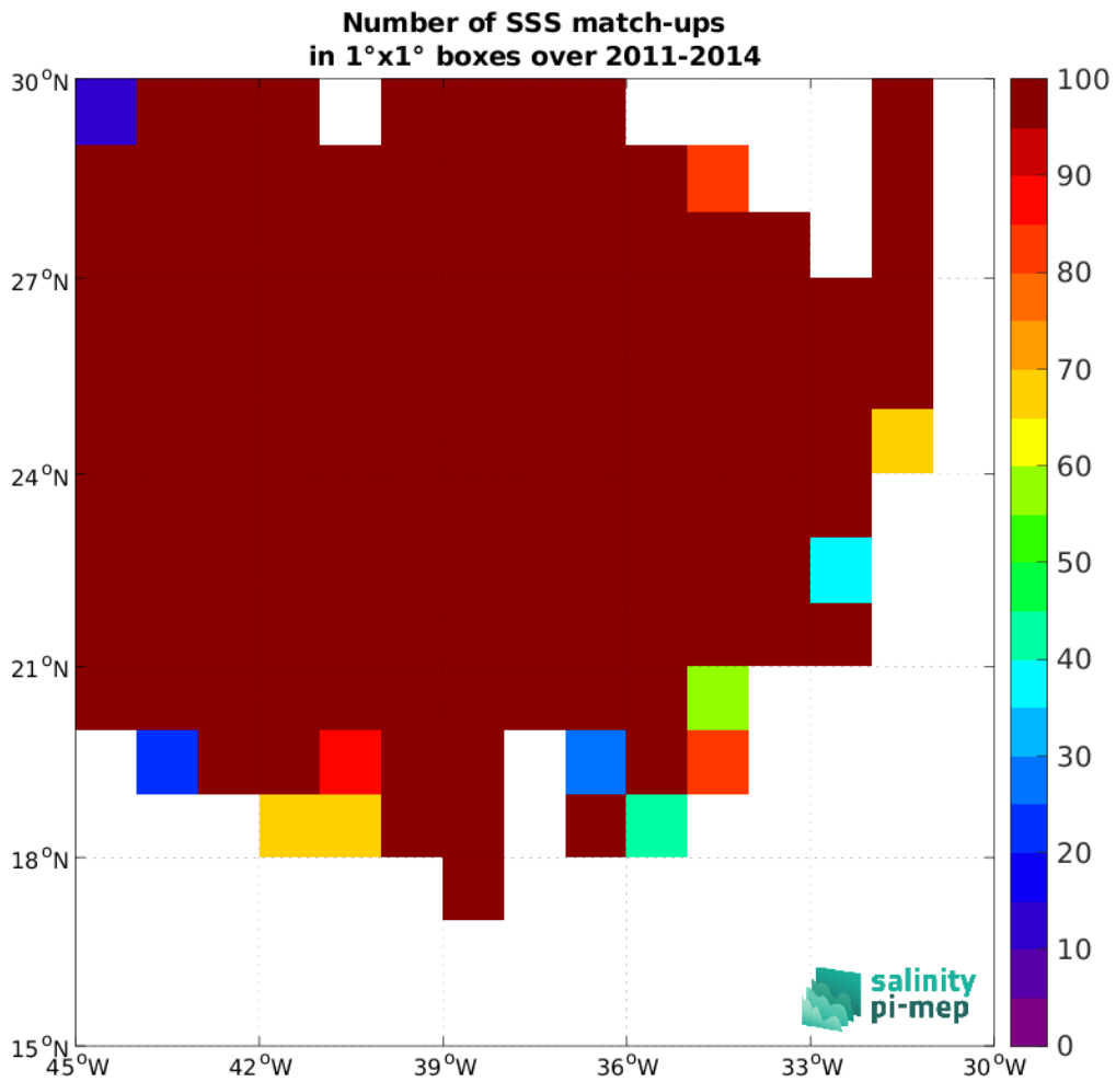
Figure 3: Number of SSS match-ups between Surface drifters SSS and the Aquarius SSS L3 OR v5 - 7-Day running (NASA-GSFC) SSS product for the SPURS 1 Pi-MEP region over 1^\circ \times 1^\circ boxes and for the full satellite product period.
