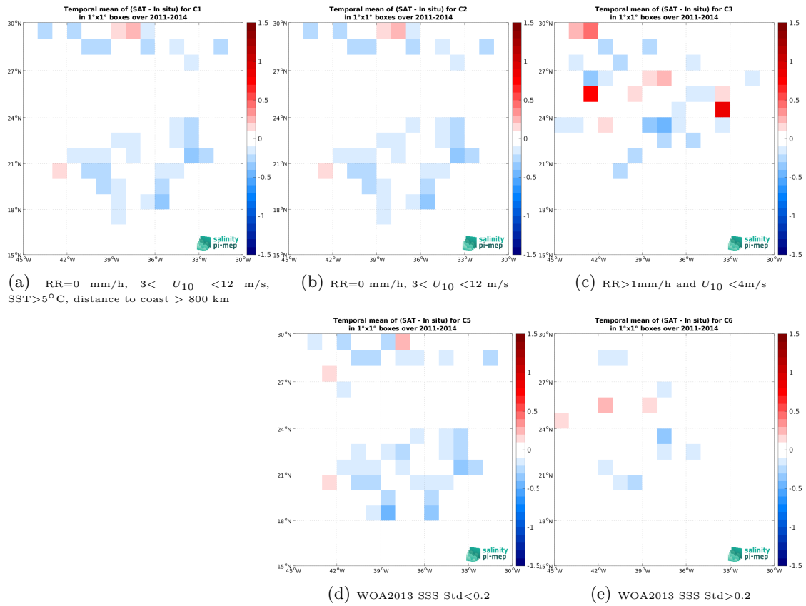
Figure 11: Temporal mean gridded over spatial boxes of size 1^\circ \times 1^\circ of \Delta\text{SSS} (Aquarius SSS L3 OR v5 - 7-Day running (NASA-GSFC) - Surface drifters) for 5 different subdatasets corresponding to:RR=0 mm/h, 3 < U_{10} < 12 m/s, SST >5^\circ\text{C} , distance to coast > 800 km (a), RR=0 mm/h, 3 < U_{10} < 12 m/s (b), RR >1 mm/h and U_{10} < 4 m/s (c), WOA2013 SSS Std <0.2 (d), WOA2013 SSS Std >0.2 (e).
