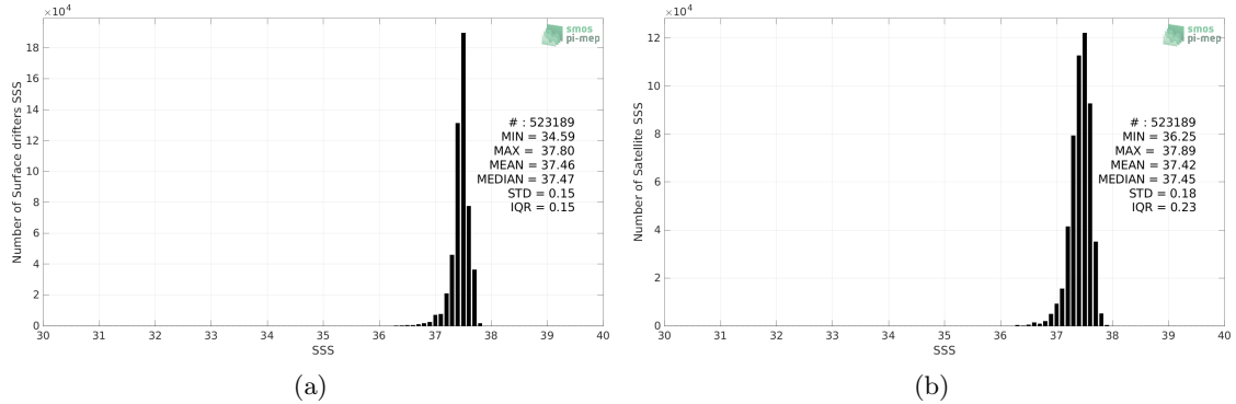
Figure 2: Histograms of SSS from Surface drifters (a) and Aquarius SSS L3 OR v5 - 7-Day running (NASA-GSFC) (b) considering all match-up pairs per bins of 0.1 over the SPURS 1 Pi-MEP region and for the full satellite product period.
