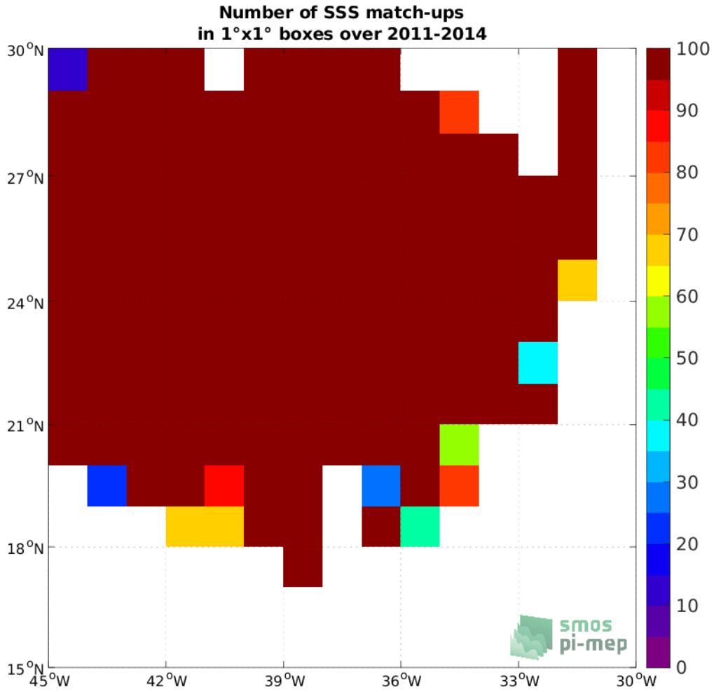
Figure 3: Number of SSS match-ups between Surface drifters SSS and the Aquarius SSS L3 OR v5 - 7-Day running (NASA-GSFC) SSS product for the SPURS 1 Pi-MEP region over 1°x1° boxes and for the full satellite product period.
