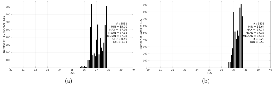
Figure 3: Histograms of SSS from TSG (SAMOS) (a) and Aquarius SSS L3 OR v5 - 7-Day running - Rain mask (NASA-GSFC) (b) considering all match-up pairs per bins of 0.1 over the SPURS 1 Pi-MEP region and for the full satellite product period.
