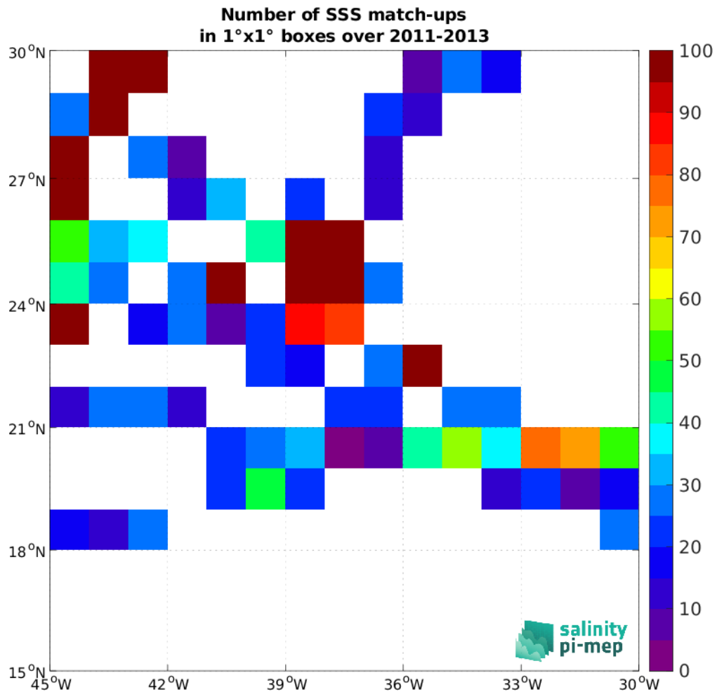
Figure 5: Number of SSS match-ups between TSG (SAMOS) SSS and the Aquarius SSS L3 OR v5 - 7-Day running - Rain mask (NASA-GSFC) SSS product for the SPURS 1 Pi-MEP region over 1^\circ \times 1^\circ boxes and for the full satellite product period.
