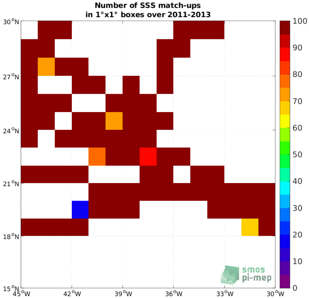
Figure 4: Number of SSS match-ups between TSG (SAMOS) SSS and the Aquarius SSS L3 OR v5 - 7-Day running - Rain mask (NASA-GSFC) SSS product for the SPURS 1 Pi-MEP region over 1°x1° boxes and for the full satellite product period.
