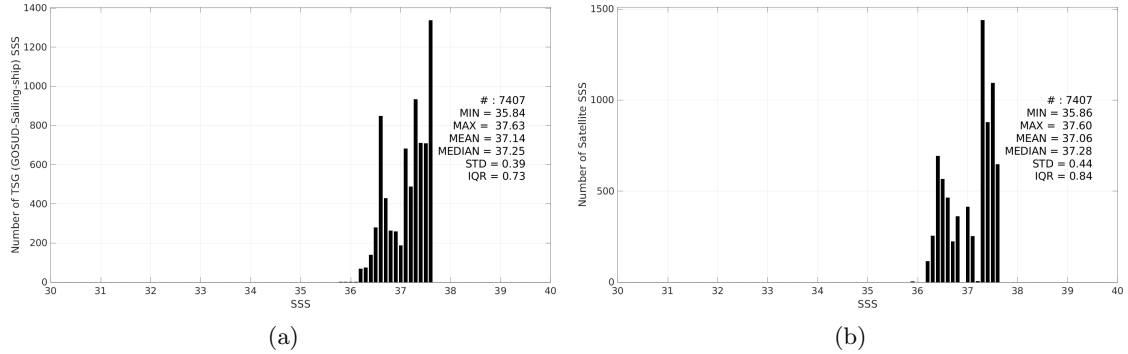
Figure 3: Histograms of SSS from TSG (GOSUD-Sailing-ship) (a) and Aquarius SSS L3 OR v5 - 7-Day running - Rain mask (NASA-GSFC) (b) considering all match-up pairs per bins of 0.1 over the SPURS 1 Pi-MEP region and for the full satellite product period.
