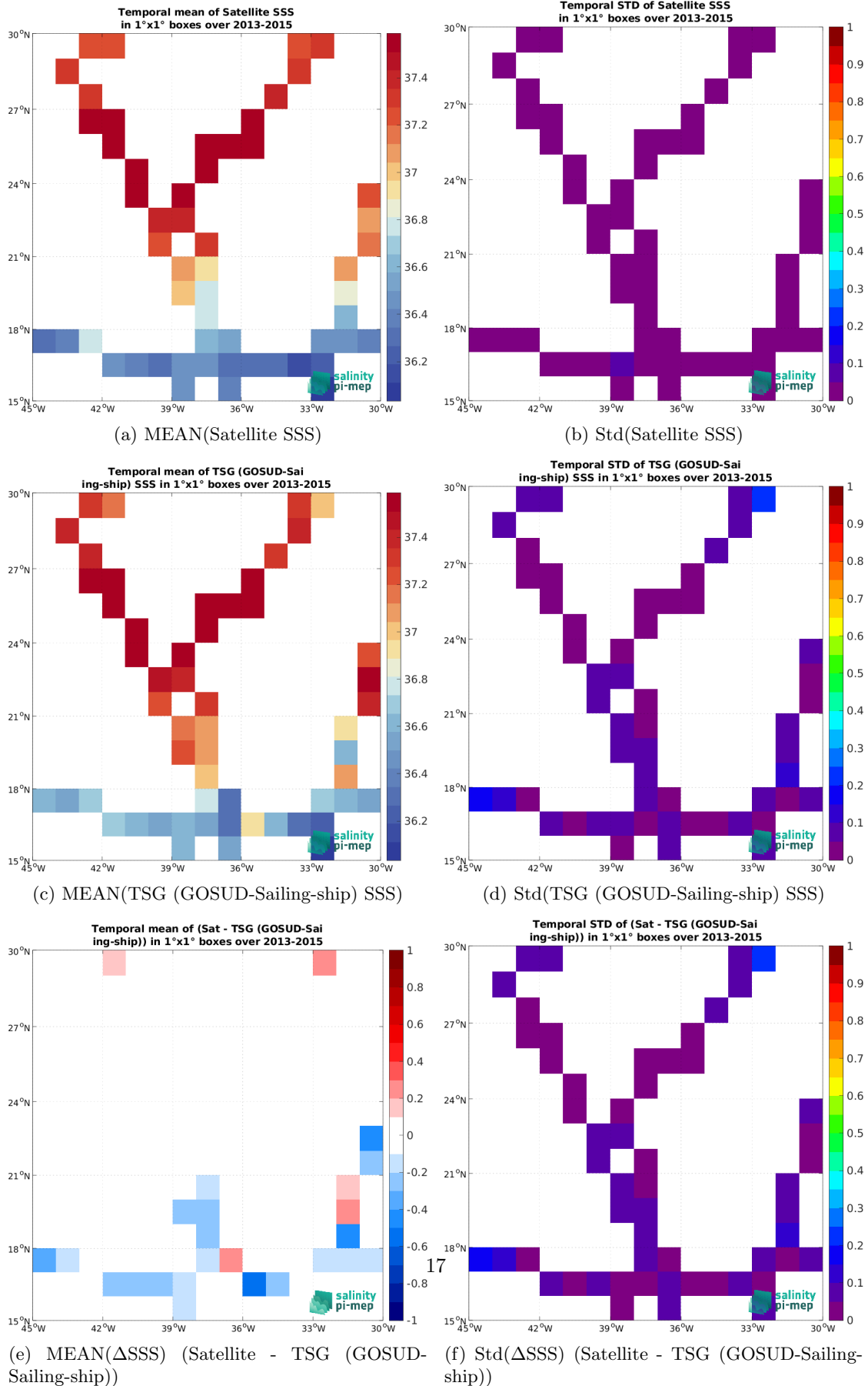
Figure 7: Temporal mean (left) and Std (right) of SSS from Aquarius SSS L3 OR v5 - 7-Day running - Rain mask (NASA-GSFC) (top), TSG (GOSUD-Sailing-ship) (middle), and of \Delta SSS (Satellite - TSG (GOSUD-Sailing-ship)). Only match-up pairs are used to generate these maps.
