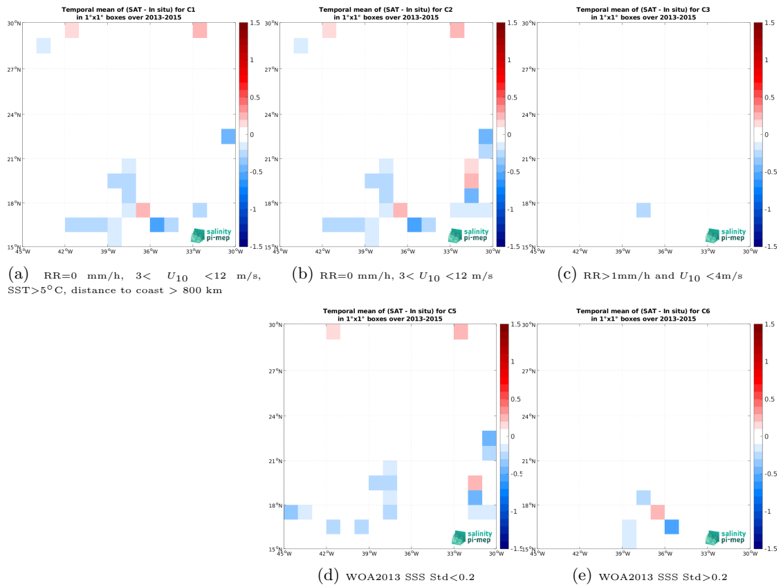
Figure 14: Temporal mean gridded over spatial boxes of size 1^\circ \times 1^\circ of \Delta SSS (Aquarius SSS L3 OR v5 - 7-Day running - Rain mask (NASA-GSFC) - TSG (GOSUD-Sailing-ship)) for 5 different subdatasets corresponding to:RR=0 mm/h, 3 < U_{10} < 12 m/s, SST >5^\circ C, distance to coast > 800 km (a), RR=0 mm/h, 3 < U_{10} < 12 m/s (b), RR >1 mm/h and U_{10} < 4 m/s (c), WOA2013 SSS Std <0.2 (d), WOA2013 SSS Std >0.2 (e).
