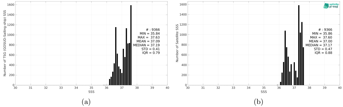
Figure 2: Histograms of SSS from TSG (GOSUD-Sailing-ship) (a) and Aquarius SSS L3 OR v5 - 7-Day running - Rain mask (NASA-GSFC) (b) considering all match-up pairs per bins of 0.1 over the SPURS 1 Pi-MEP region and for the full satellite product period.
