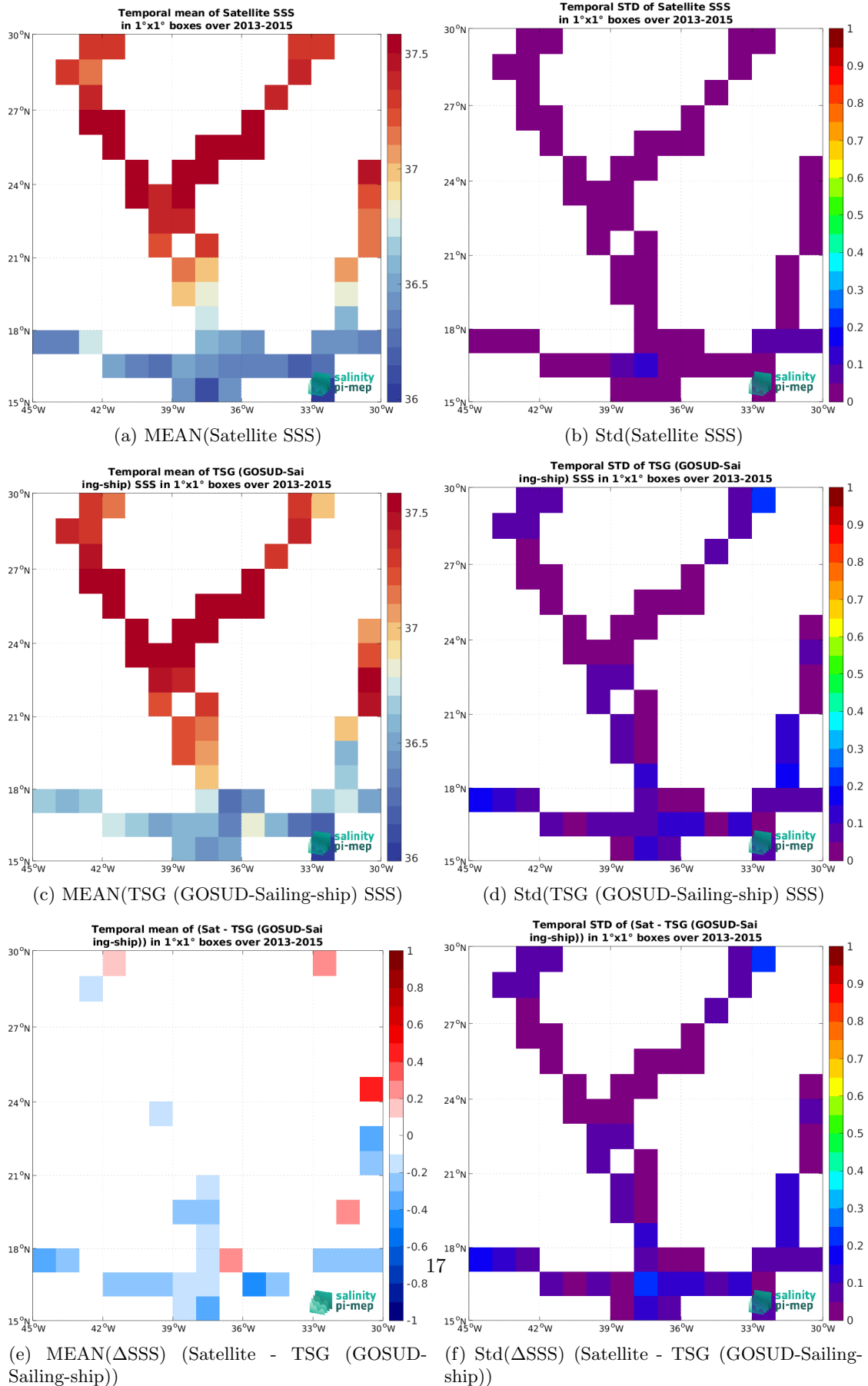
Figure 6: Temporal mean (left) and Std (right) of SSS from Aquarius SSS L3 OR v5 - 7-Day running - Rain mask (NASA-GSFC) (top), TSG (GOSUD-Sailing-ship) (middle), and of \Delta SSS (Satellite - TSG (GOSUD-Sailing-ship)). Only match-up pairs are used to generate these maps.
