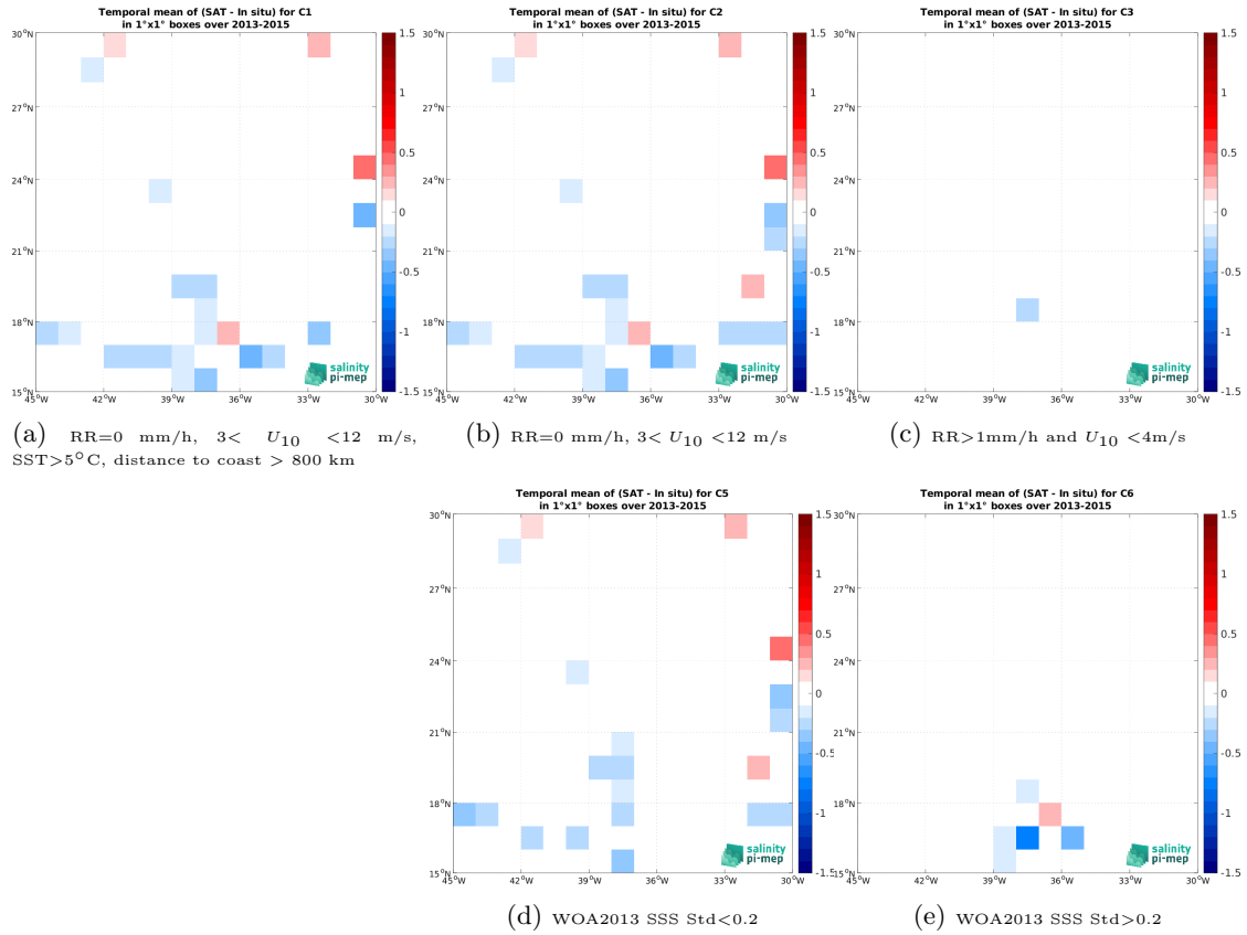
Figure 12: Temporal mean gridded over spatial boxes of size 1^{\circ} \times 1^{\circ} of \Delta\text{SSS} (Aquarius SSS L3 OR v5 - 7-Day running - Rain mask (NASA-GSFC) - TSG (GOSUD-Sailing-ship)) for 5 different subdatasets corresponding to: RR=0 mm/h, 3 < U_{10} < 12 m/s, SST > 5^{\circ}\text{C} , distance to coast > 800 km (a), RR=0 mm/h, 3 < U_{10} < 12 m/s (b), RR > 1\text{mm/h} and U_{10} < 4\text{m/s} (c), WOA2013 SSS Std < 0.2 (d), WOA2013 SSS Std > 0.2 (e).
