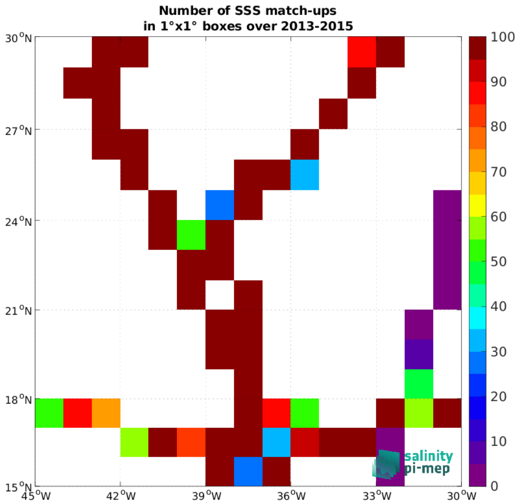
Figure 4: Number of SSS match-ups between TSG (GOSUD-Sailing-ship) SSS and the Aquarius SSS L3 OR v5 - 7-Day running - Rain mask (NASA-GSFC) SSS product for the SPURS 1 Pi-MEP region over 1°x1° boxes and for the full satellite product period.
