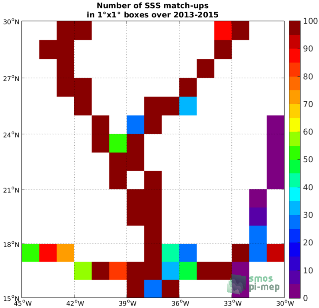
Figure 4: Number of SSS match-ups between TSG (GOSUD-Sailing-ship) SSS and the Aquarius SSS L3 OR v5 - 7-Day running - Rain mask (NASA-GSFC) SSS product for the SPURS 1 Pi-MEP region over 1^\circ \times 1^\circ boxes and for the full satellite product period.
