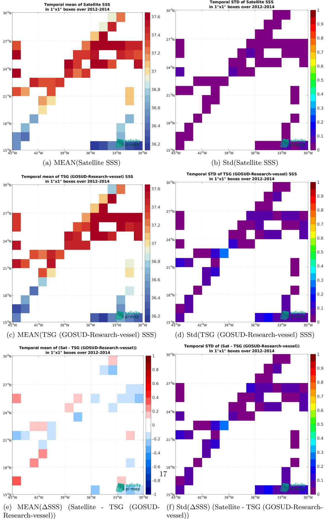
Figure 7: Temporal mean (left) and Std (right) of SSS from Aquarius SSS L3 OR v5 - 7-Day running - Rain mask (NASA-GSFC) (top), TSG (GOSUD-Research-vessel) (middle), and of \Delta SSS (Satellite - TSG (GOSUD-Research-vessel)). Only match-up pairs are used to generate these maps.
