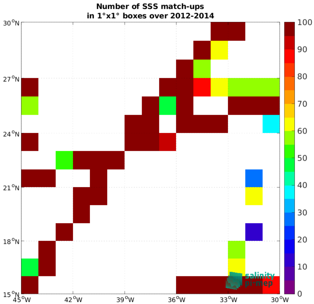
Figure 5: Number of SSS match-ups between TSG (GOSUD-Research-vessel) SSS and the Aquarius SSS L3 OR v5 - 7-Day running - Rain mask (NASA-GSFC) SSS product for the SPURS 1 Pi-MEP region over 1°x1° boxes and for the full satellite product period.
