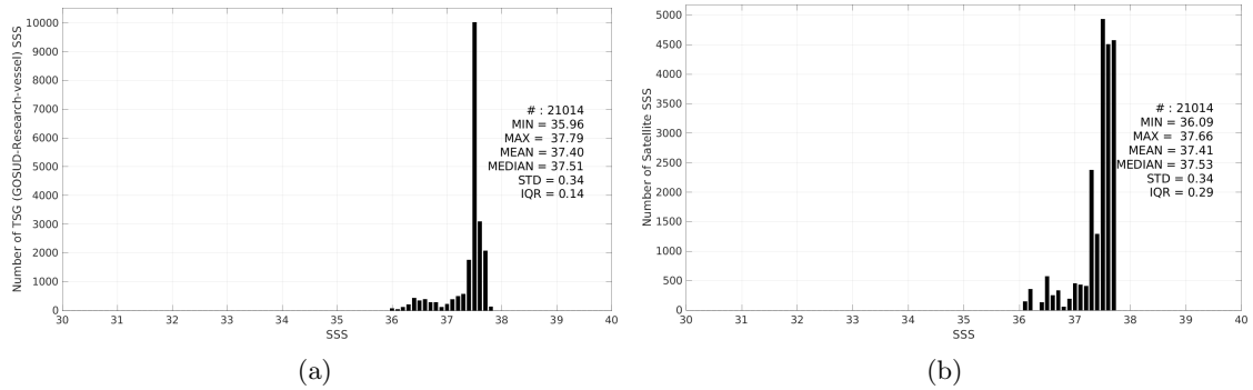
Figure 3: Histograms of SSS from TSG (GOSUD-Research-vessel) (a) and Aquarius SSS L3 OR v5 - 7-Day running - Rain mask (NASA-GSFC) (b) considering all match-up pairs per bins of 0.1 over the SPURS 1 Pi-MEP region and for the full satellite product period.
