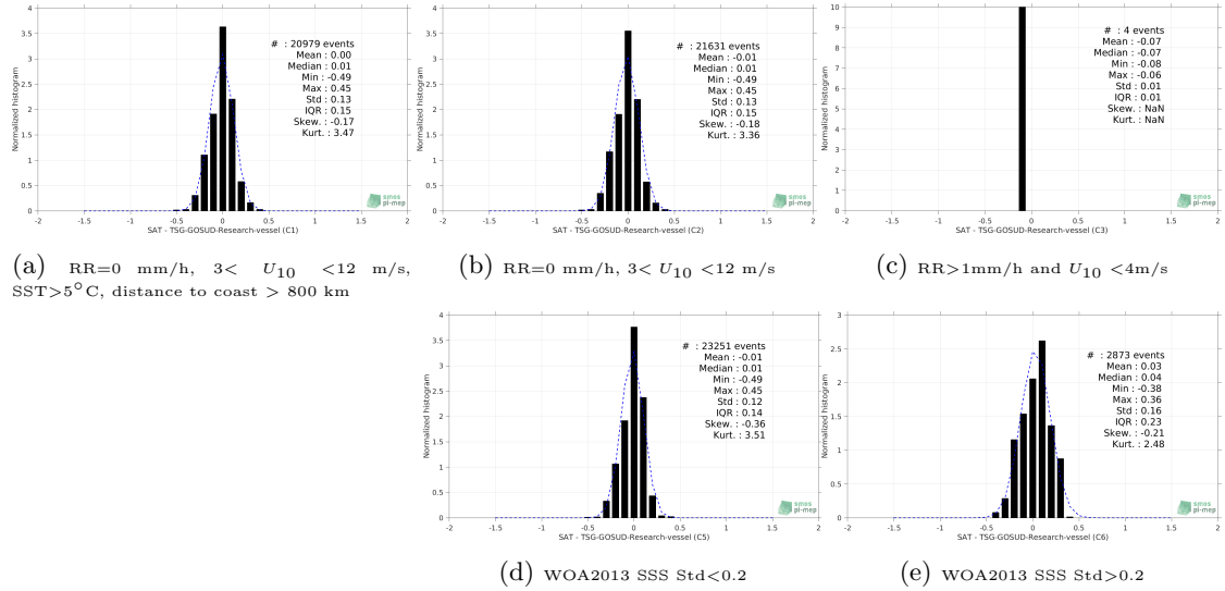
Figure 13: Normalized histogram of \Delta\text{SSS} (Aquarius-L3-OR-V5-7DAY-RUNNING-RAIN-MASK-1DEG - TSG-GOSUD-Research-vessel) for 5 different subdatasets corresponding to: RR=0 mm/h, 3 < U_{10} < 12 m/s, SST > 5^{\circ}\text{C} , distance to coast > 800 km (a), RR=0 mm/h, 3 < U_{10} < 12 m/s (b), RR > 1\text{mm/h} and U_{10} < 4\text{m/s} (c), WOA2013 SSS Std < 0.2 (d), WOA2013 SSS Std > 0.2 (e).
