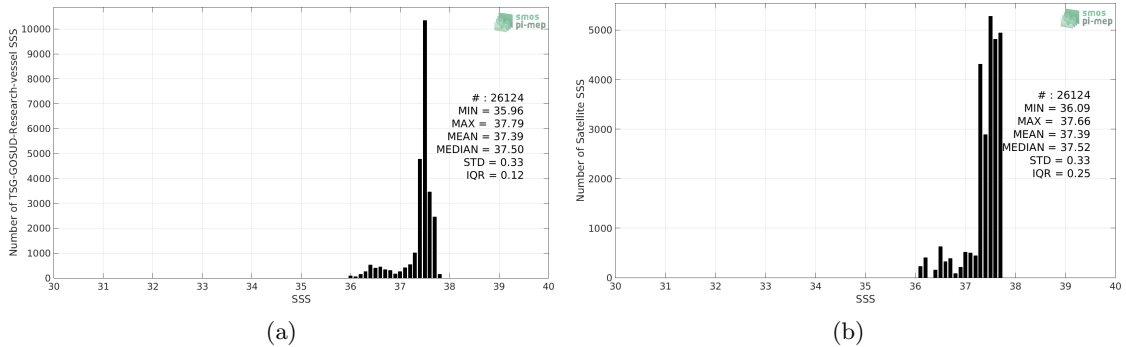
Figure 2: Histograms of SSS from TSG-GOSUD-Research-vessel (a) and Aquarius-L3-OR-V5-7DAY-RUNNING-RAIN-MASK-1DEG (b) considering all match-up pairs per bins of 0.1 over the SPURS 1 Pi-MEP region and for the full satellite product period.
