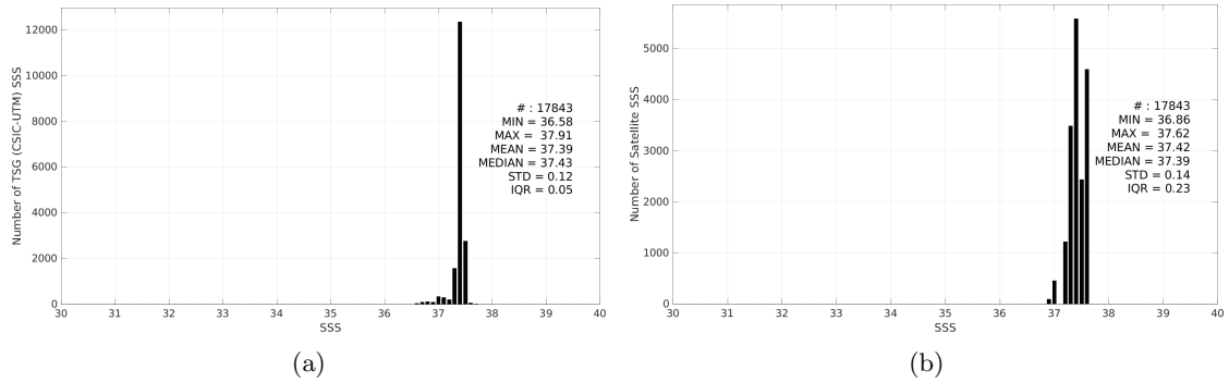
Figure 3: Histograms of SSS from TSG (CSIC-UTM) (a) and Aquarius SSS L3 OR v5 - 7-Day running - Rain mask (NASA-GSFC) (b) considering all match-up pairs per bins of 0.1 over the SPURS 1 Pi-MEP region and for the full satellite product period.
