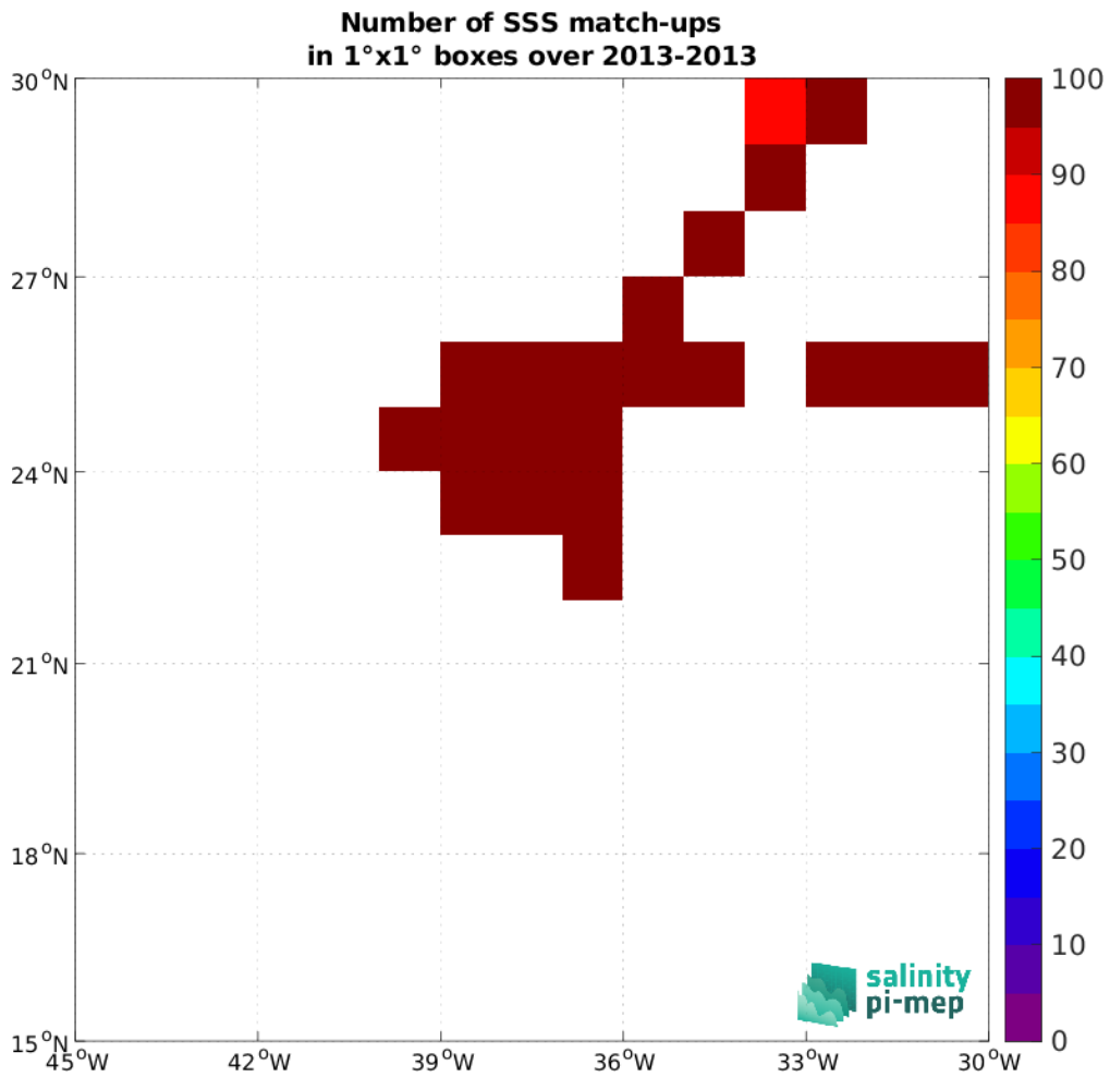
Figure 5: Number of SSS match-ups between TSG (CSIC-UTM) SSS and the Aquarius SSS L3 OR v5 - 7-Day running - Rain mask (NASA-GSFC) SSS product for the SPURS 1 Pi-MEP region over 1^\circ \times 1^\circ boxes and for the full satellite product period.
