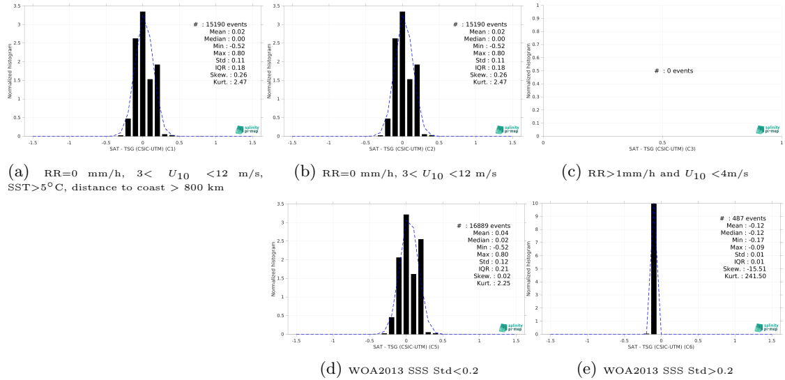
Figure 15: Normalized histogram of \Delta SSS (Aquarius SSS L3 OR v5 - 7-Day running - Rain mask (NASA-GSFC) - TSG (CSIC-UTM)) for 5 different subdatasets corresponding to: RR=0 mm/h, 3 < U_{10} < 12 m/s, SST > 5°C, distance to coast > 800 km (a), RR=0 mm/h, 3 < U_{10} < 12 m/s (b), RR > 1mm/h and U_{10} < 4 m/s (c), WOA2013 SSS Std < 0.2 (d), WOA2013 SSS Std > 0.2 (e).
