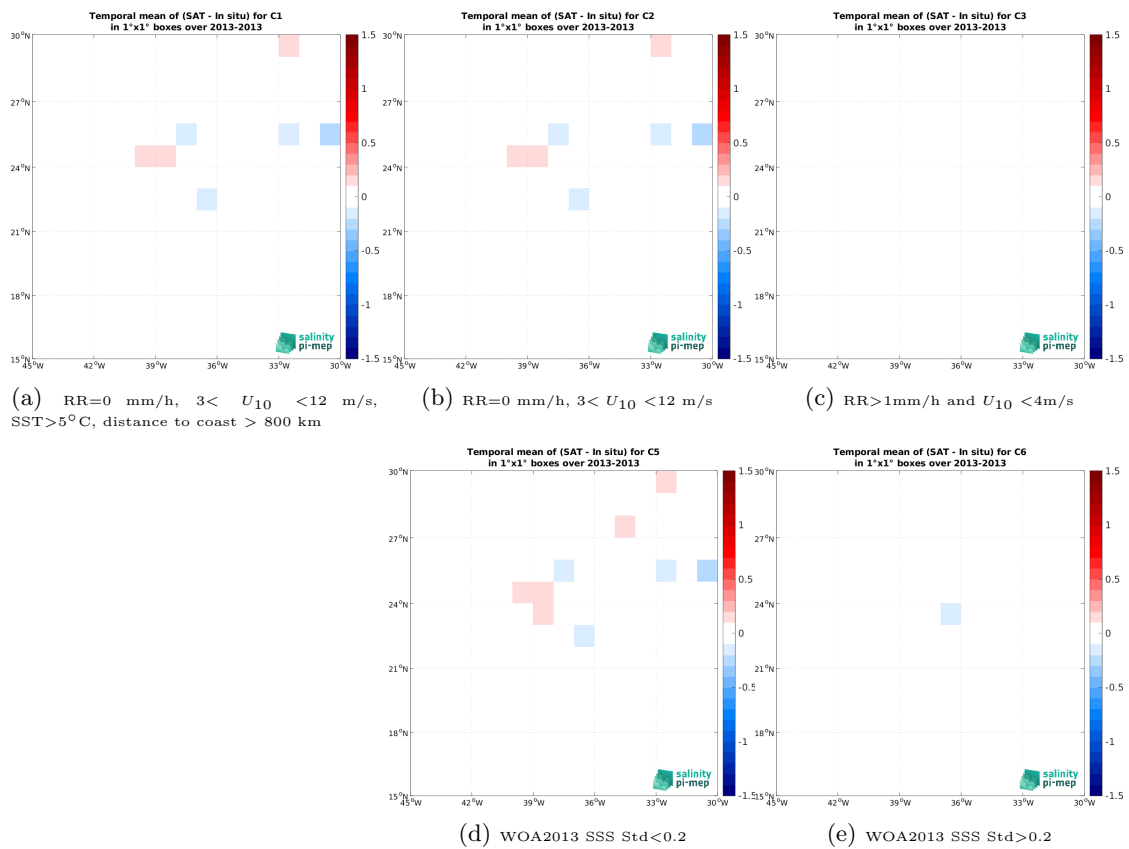
Figure 14: Temporal mean gridded over spatial boxes of size 1^\circ \times 1^\circ of \Delta SSS (Aquarius SSS L3 OR v5 - 7-Day running - Rain mask (NASA-GSFC) - TSG (CSIC-UTM)) for 5 different subdatasets corresponding to:RR=0 mm/h, 3 < U_{10} < 12 m/s, SST>5°C, distance to coast > 800 km (a), RR=0 mm/h, 3 < U_{10} < 12 m/s (b), RR>1mm/h and U_{10} < 4 m/s (c), WOA2013 SSS Std<0.2 (d), WOA2013 SSS Std>0.2 (e).
