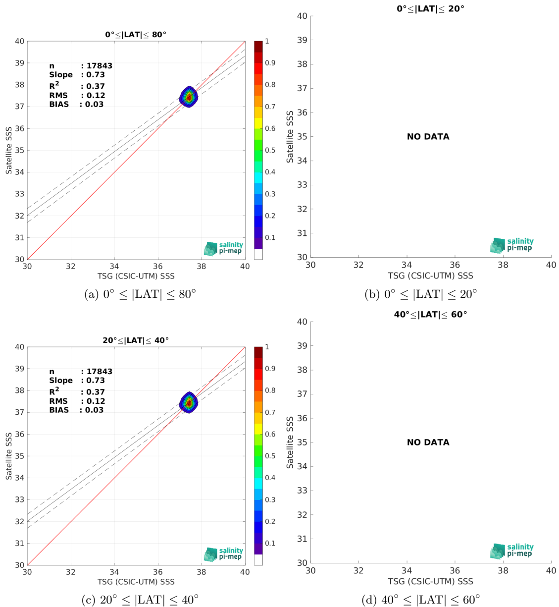
Figure 10: Contour maps of the concentration of Aquarius SSS L3 OR v5 - 7-Day running - Rain mask (NASA-GSFC) SSS (y-axis) versus TSG (CSIC-UTM) SSS (x-axis) at match-up pairs for different latitude bands. For each plot, the red line shows x=y . The black thin and dashed lines indicate a linear fit through the data cloud and the \pm 95\% confidence levels, respectively. The number match-up pairs n , the slope and R^2 coefficient of the linear fit, the root mean square (RMS) and the mean bias between satellite and in situ data are indicated for each latitude band in each plots.
