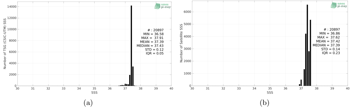
Figure 2: Histograms of SSS from TSG (CSIC-UTM) (a) and Aquarius SSS L3 OR v5 - 7-Day running - Rain mask (NASA-GSFC) (b) considering all match-up pairs per bins of 0.1 over the SPURS 1 Pi-MEP region and for the full satellite product period.
