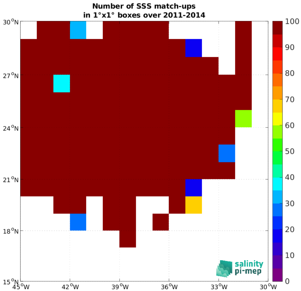
Figure 4: Number of SSS match-ups between Surface drifters SSS and the Aquarius SSS L3 OR v5 - 7-Day running - Rain mask (NASA-GSFC) SSS product for the SPURS 1 Pi-MEP region over 1°x1° boxes and for the full satellite product period.
