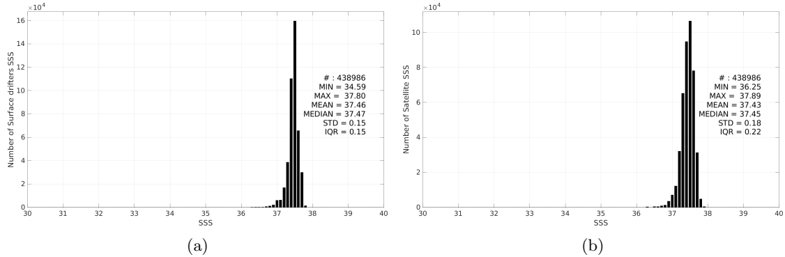
Figure 3: Histograms of SSS from Surface drifters (a) and Aquarius SSS L3 OR v5 - 7-Day running - Rain mask (NASA-GSFC) (b) considering all match-up pairs per bins of 0.1 over the SPURS 1 Pi-MEP region and for the full satellite product period.
