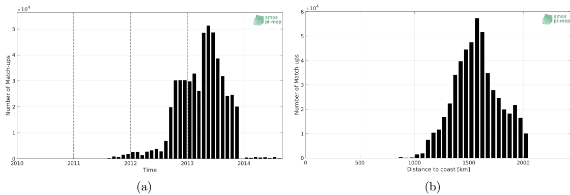
Figure 1: Number of match-ups between Surface drifters and Aquarius SSS L3 OR v5 - 7-Day running - Rain mask (NASA-GSFC) SSS as a function of time (a) and as function of the distance to coast (b) over the SPURS 1 Pi-MEP region and for the full satellite product period.
