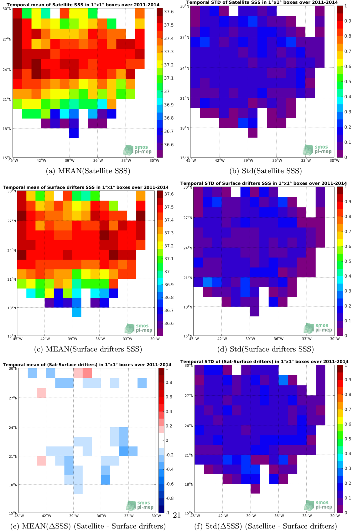
Figure 5: Temporal mean (left) and Std (right) of SSS from Aquarius-L3-OR-V5-7DAY-RUNNING-RAIN-MASK-1DEG (top), Surface drifters (middle), and of \Delta SSS (Satellite - Surface drifters). Only match-up pairs are used to generate these maps.
