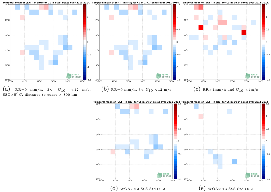
Figure 11: Temporal mean gridded over spatial boxes of size 1^\circ \times 1^\circ of \Delta SSS (Aquarius-L3-OR-V5-7DAY-RUNNING-RAIN-MASK-1DEG - Surface drifters) for 5 different subdatasets corresponding to:RR=0 mm/h, 3 < U_{10} < 12 m/s, SST >5^\circ C, distance to coast > 800 km (a), RR=0 mm/h, 3 < U_{10} < 12 m/s (b), RR >1 mm/h and U_{10} < 4 m/s (c), WOA2013 SSS Std <0.2 (d), WOA2013 SSS Std >0.2 (e).
