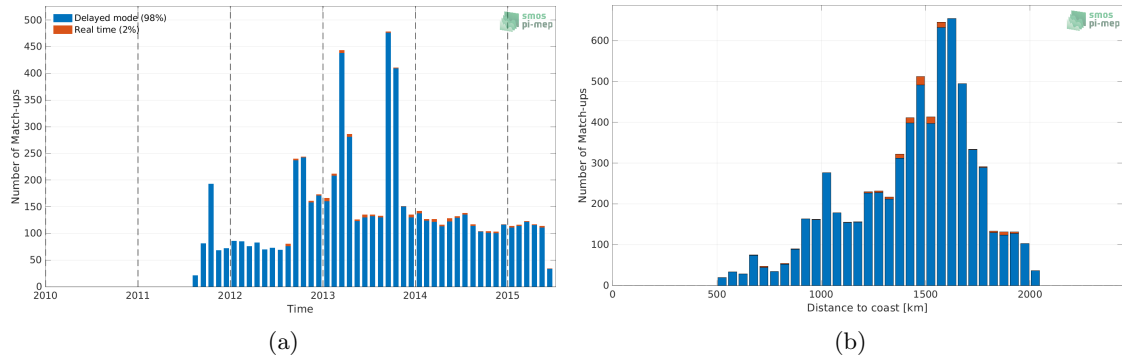
Figure 1: Number of match-ups between Argo and Aquarius SSS L3 OR v5 - 7-Day running - Rain mask (NASA-GSFC) SSS as a function of time (a) and as function of the distance to coast (b) over the SPURS 1 Pi-MEP region and for the full satellite product period.
