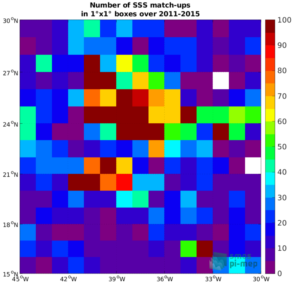
Figure 4: Number of SSS match-ups between Argo SSS and the Aquarius SSS L3 OR v5 - 7-Day running - Rain mask (NASA-GSFC) SSS product for the SPURS 1 Pi-MEP region over 1°x1° boxes and for the full satellite product period.
