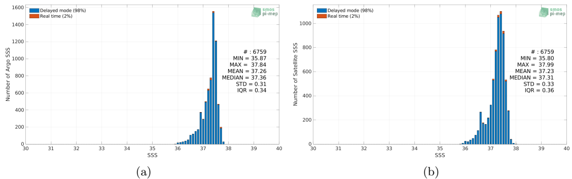
Figure 2: Histograms of SSS from Argo (a) and Aquarius SSS L3 OR v5 - 7-Day running - Rain mask (NASA-GSFC) (b) considering all match-up pairs per bins of 0.1 over the SPURS 1 Pi-MEP region and for the full satellite product period.
