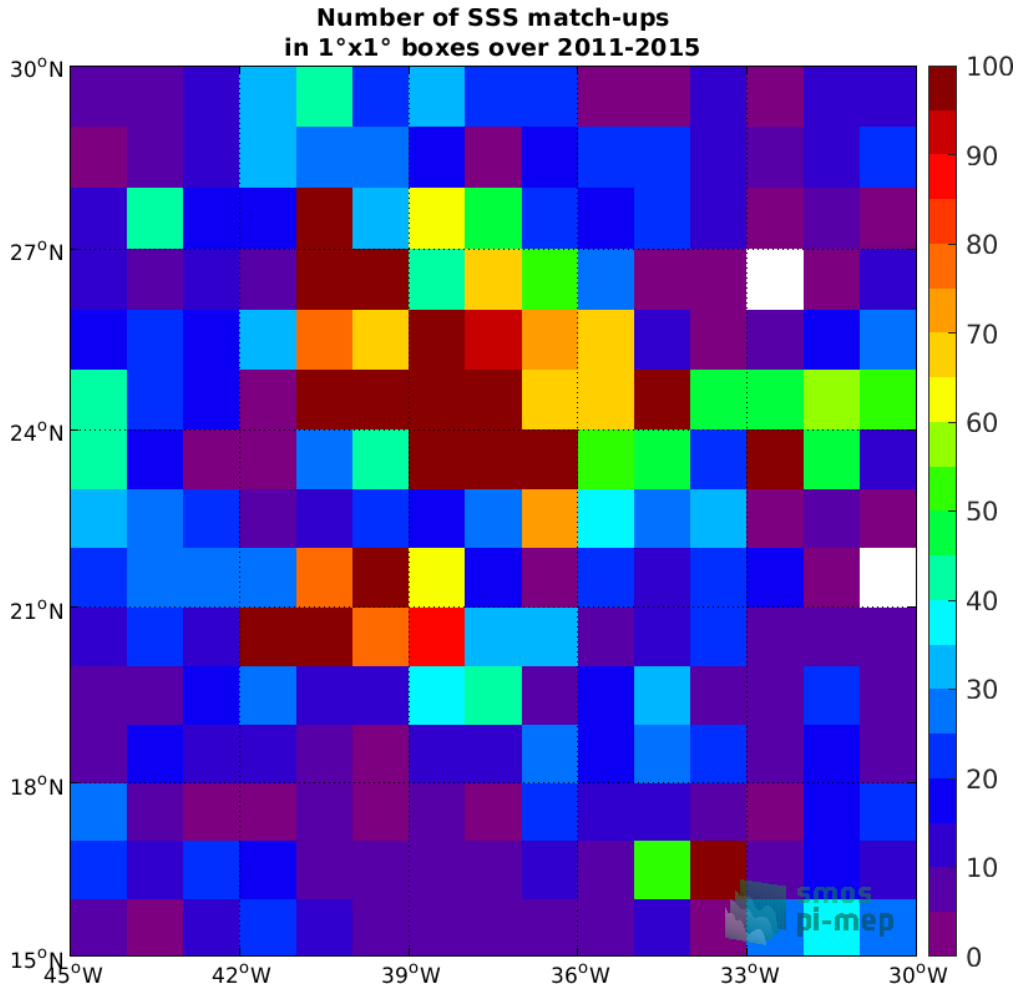
Figure 4: Number of SSS match-ups between Argo SSS and the Aquarius SSS L3 OR v5 - 7-Day running - Rain mask (NASA-GSFC) SSS product for the SPURS 1 Pi-MEP region over 1^\circ \times 1^\circ boxes and for the full satellite product period.
