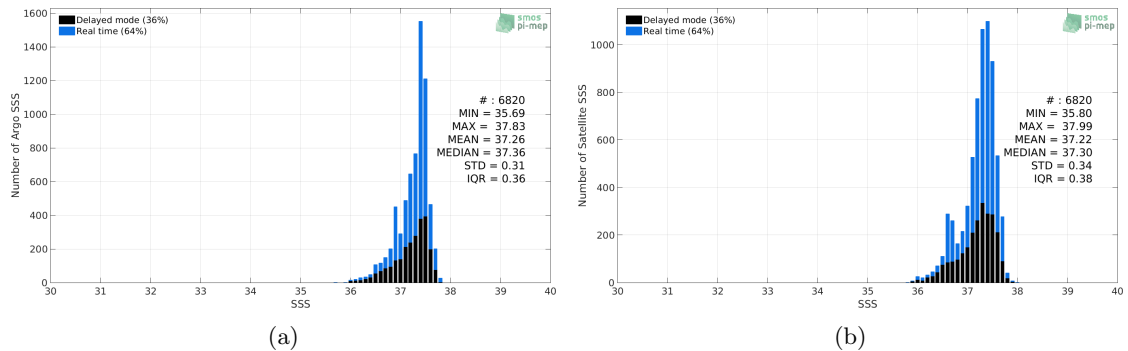
Figure 2: Histograms of SSS from Argo (a) and Aquarius-L3-OR-V5-7DAY-RUNNING-RAIN-MASK-1DEG (b) considering all match-up pairs per bins of 0.1 over the SPURS 1 Pi-MEP region and for the full satellite product period.
