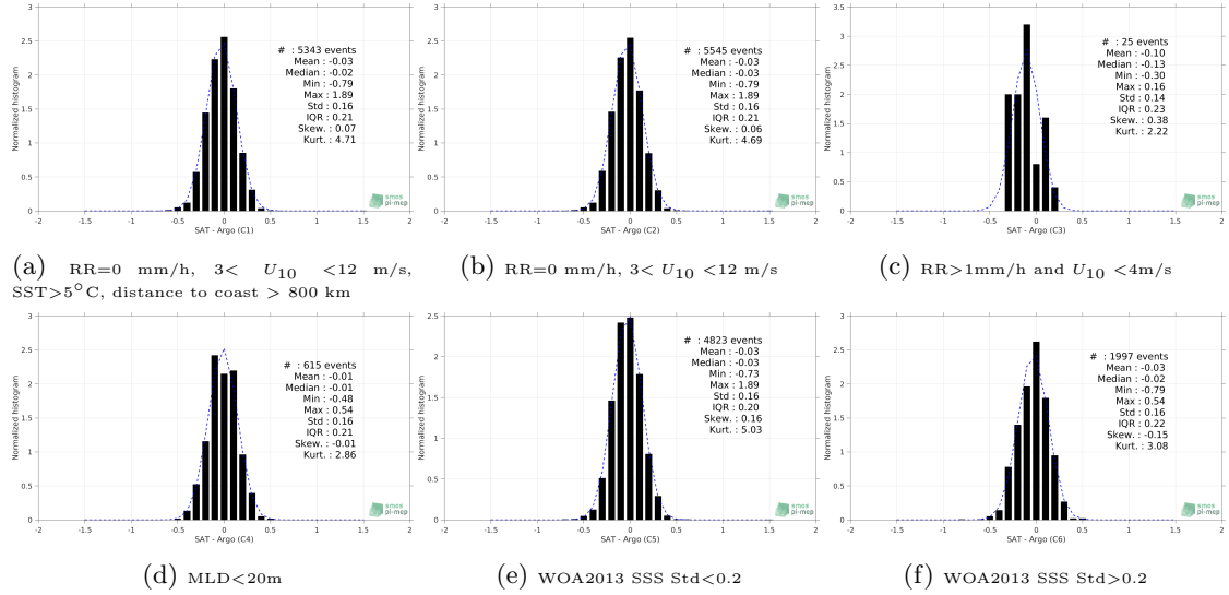
Figure 13: Normalized histogram of \Delta SSS (Aquarius-L3-OR-V5-7DAY-RUNNING-RAIN-MASK-1DEG - Argo) for 6 different subdatasets corresponding to: RR=0 mm/h, 3 < U_{10} < 12 m/s, SST > 5°C, distance to coast > 800 km (a), RR=0 mm/h, 3 < U_{10} < 12 m/s (b), RR > 1mm/h and U_{10} < 4 m/s (c), MLD < 20m (d), WOA2013 SSS Std < 0.2 (e), WOA2013 SSS Std > 0.2 (f).
