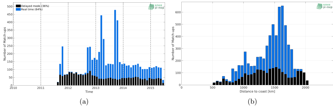
Figure 1: Number of match-ups between Argo and Aquarius-L3-OR-V5-7DAY-RUNNING-RAIN-MASK-1DEG SSS as a function of time (a) and as function of the distance to coast (b) over the SPURS 1 Pi-MEP region and for the full satellite product period.
