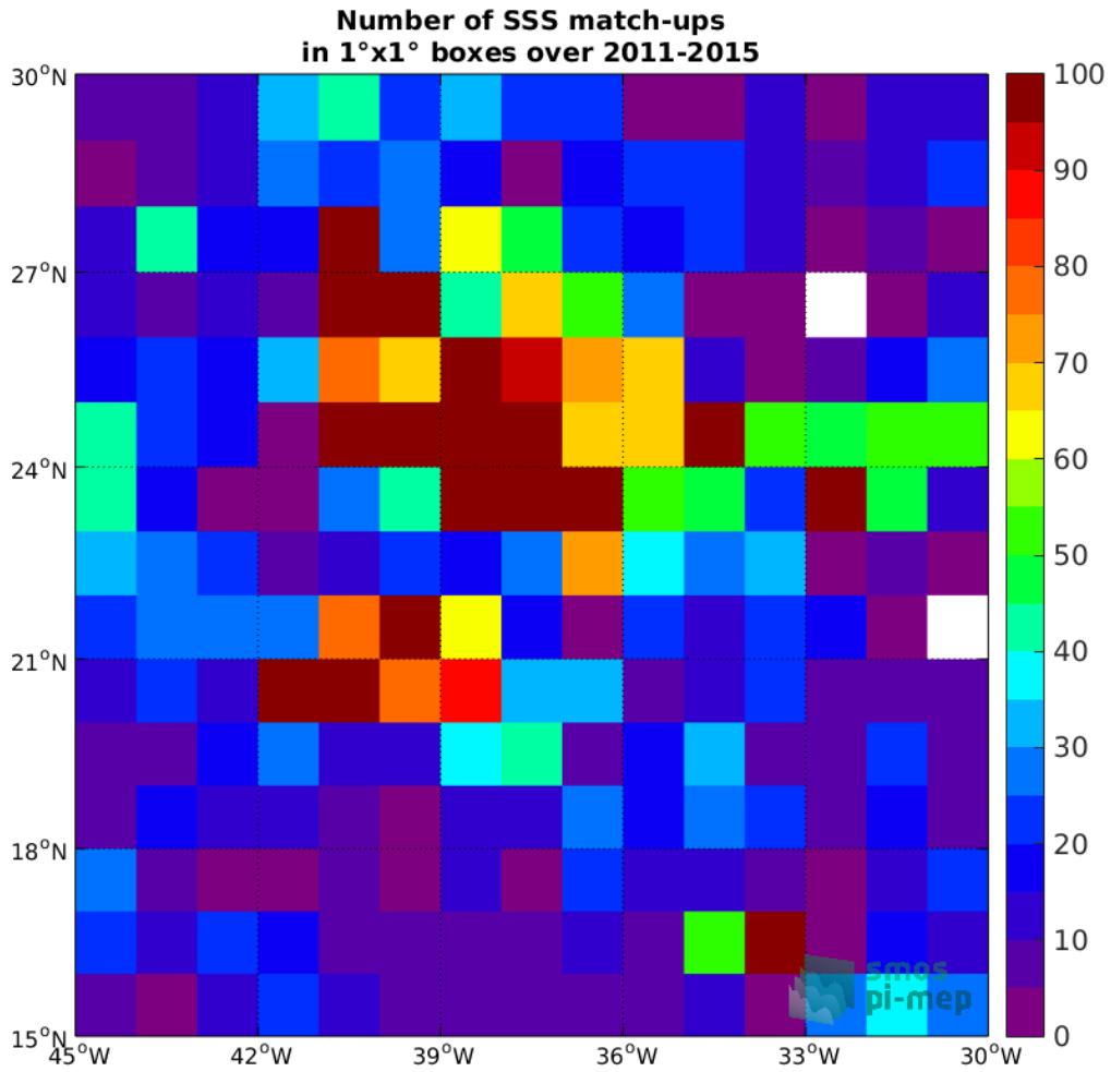
Figure 4: Number of SSS match-ups between Argo SSS and the Aquarius-L3-OR-V5-7DAY-RUNNING-RAIN-MASK-1DEG SSS product for the SPURS 1 Pi-MEP region over 1°x1° boxes and for the full satellite product period.
