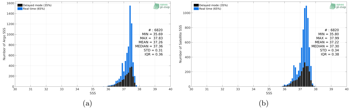
Figure 2: Histograms of SSS from Argos (a) and Aquarius-L3-OR-V5-7DAY-RUNNING-RAIN-MASK-1DEG (b) considering all match-up pairs per bins of 0.1 over the SPURS 1 Pi-MEP region and for the full satellite product period.
