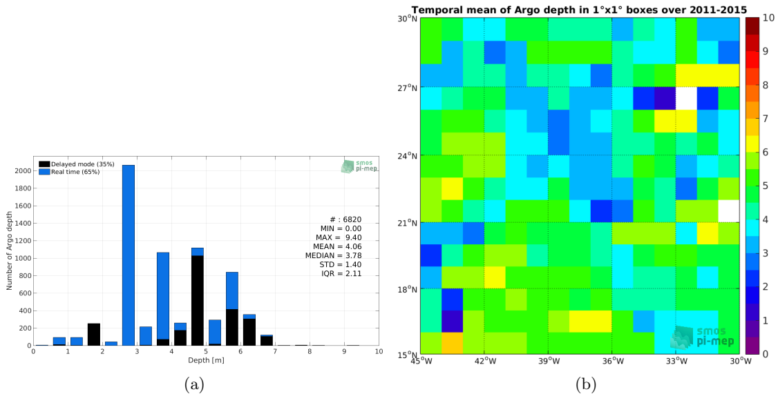
Figure 3: Histograms of the depth of the upper level SSS measurements from Argos in the Match-up DataBase for the SPURS 1 Pi-MEP region (a) and temporal mean spatial distribution of pressure of the in situ SSS data over 1^\circ \times 1^\circ boxes and for the full satellite product period (b).
