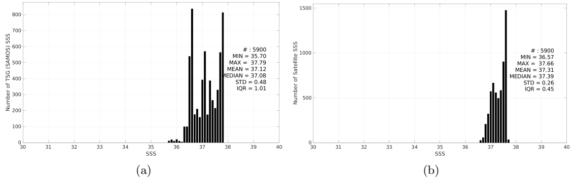
Figure 3: Histograms of SSS from TSG (SAMOS) (a) and Aquarius SSS L3 OR v5 - Monthly (NASA-GSFC) (b) considering all match-up pairs per bins of 0.1 over the SPURS 1 Pi-MEP region and for the full satellite product period.
