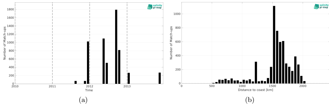
Figure 2: Number of match-ups between TSG (SAMOS) and Aquarius SSS L3 OR v5 - Monthly (NASA-GSFC) SSS as a function of time (a) and as function of the distance to coast (b) over the SPURS 1 Pi-MEP region and for the full satellite product period.
