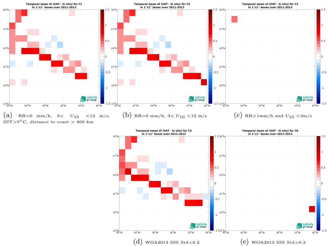
Figure 14: Temporal mean gridded over spatial boxes of size 1^\circ \times 1^\circ of \Delta SSS (Aquarius SSS L3 OR v5 - Monthly (NASA-GSFC) - TSG (SAMOS)) for 5 different subdatasets corresponding to: RR=0 mm/h, 3 < U_{10} < 12 m/s, SST > 5^\circ C , distance to coast > 800 km (a), RR=0 mm/h, 3 < U_{10} < 12 m/s (b), RR > 1 mm/h and U_{10} < 4 m/s (c), WOA2013 SSS Std < 0.2 (d), WOA2013 SSS Std > 0.2 (e).
