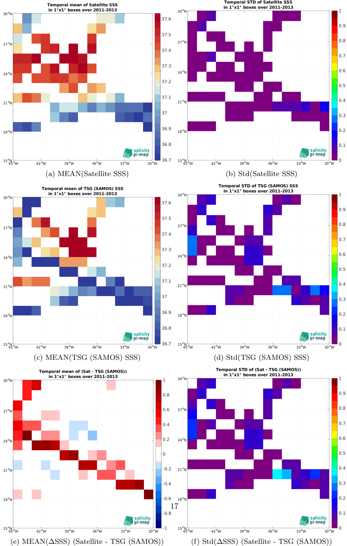
Figure 7: Temporal mean (left) and Std (right) of SSS from Aquarius SSS L3 OR v5 - Monthly (NASA-GSFC) (top), TSG (SAMOS) (middle), and of \Delta SSS (Satellite - TSG (SAMOS)). Only match-up pairs are used to generate these maps.
