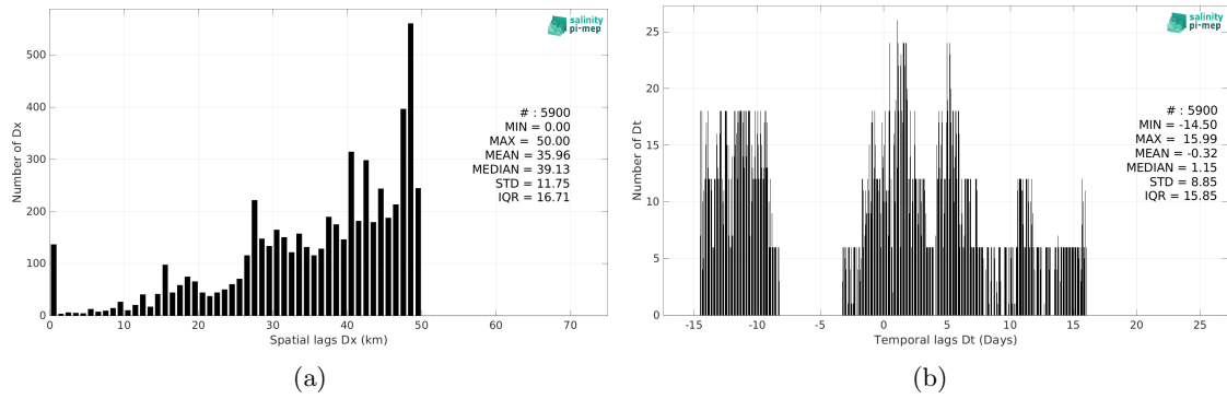
Figure 6: Histograms of the spatial (a) and temporal (b) lags between the location/time of the TSG (SAMOS) measurement and the date of the corresponding Aquarius SSS L3 OR v5 - Monthly (NASA-GSFC) SSS pixel.
