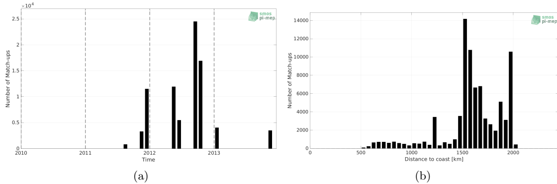
Figure 1: Number of match-ups between TSG (SAMOS) and Aquarius SSS L3 OR v5 - Monthly (NASA-GSFC) SSS as a function of time (a) and as function of the distance to coast (b) over the SPURS 1 Pi-MEP region and for the full satellite product period.
