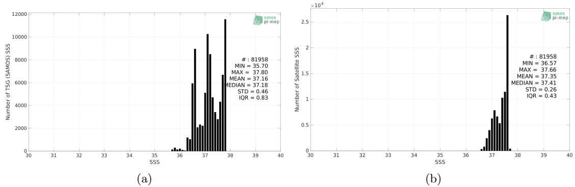
Figure 2: Histograms of SSS from TSG (SAMOS) (a) and Aquarius SSS L3 OR v5 - Monthly (NASA-GSFC) (b) considering all match-up pairs per bins of 0.1 over the SPURS 1 Pi-MEP region and for the full satellite product period.
