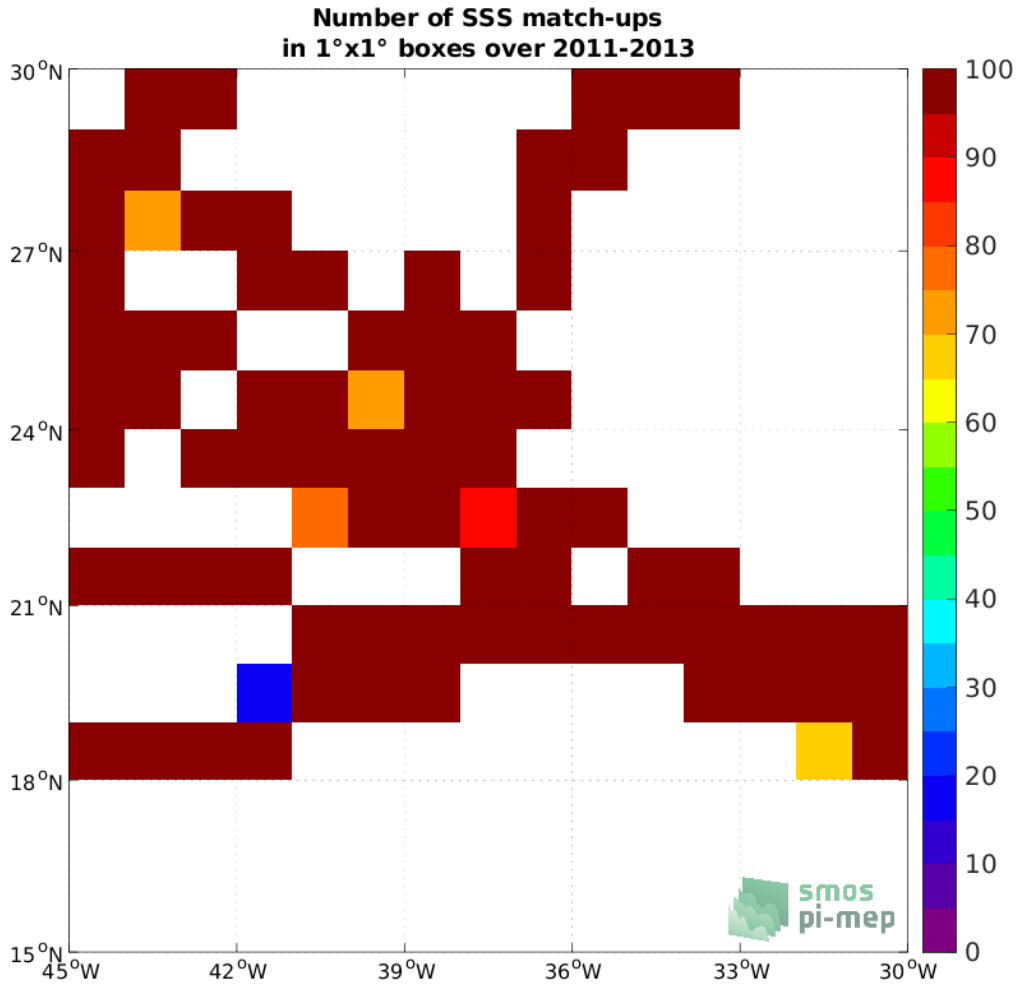
Figure 4: Number of SSS match-ups between TSG (SAMOS) SSS and the Aquarius SSS L3 OR v5 - Monthly (NASA-GSFC) SSS product for the SPURS 1 Pi-MEP region over 1°x1° boxes and for the full satellite product period.
