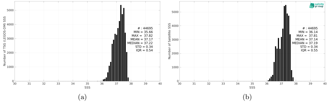
Figure 2: Histograms of SSS from TSG (LEGOS-DM) (a) and Aquarius SSS L3 OR v5 - Monthly (NASA-GSFC) (b) considering all match-up pairs per bins of 0.1 over the SPURS 1 Pi-MEP region and for the full satellite product period.
