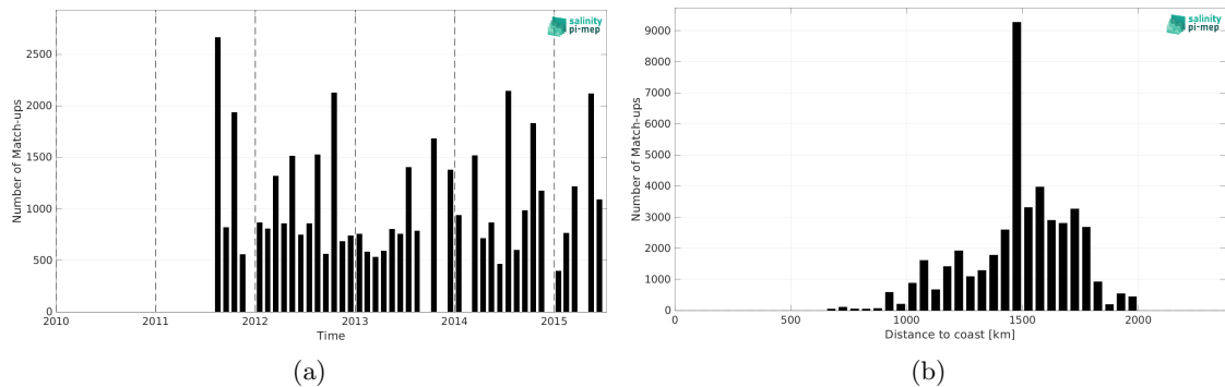
Figure 1: Number of match-ups between TSG (LEGOS-DM) and Aquarius SSS L3 OR v5 - Monthly (NASA-GSFC) SSS as a function of time (a) and as function of the distance to coast (b) over the SPURS 1 Pi-MEP region and for the full satellite product period.
