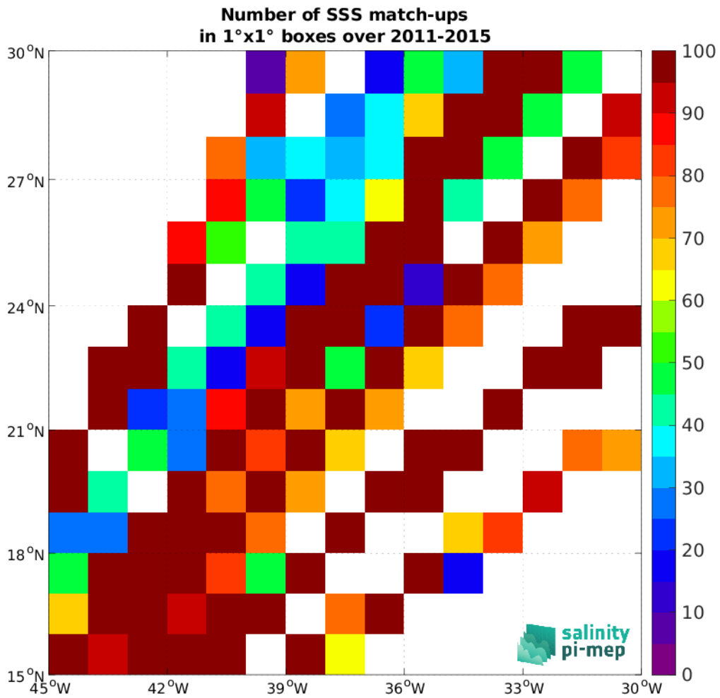
Figure 4: Number of SSS match-ups between TSG (LEGOS-DM) SSS and the Aquarius SSS L3 OR v5 - Monthly (NASA-GSFC) SSS product for the SPURS 1 Pi-MEP region over 1°x1° boxes and for the full satellite product period.
