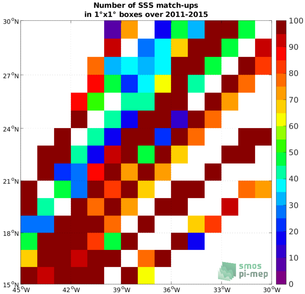
Figure 4: Number of SSS match-ups between TSG (LEGOS-DM) SSS and the Aquarius SSS L3 OR v5 - Monthly (NASA-GSFC) SSS product for the SPURS 1 Pi-MEP region over 1^\circ \times 1^\circ boxes and for the full satellite product period.
