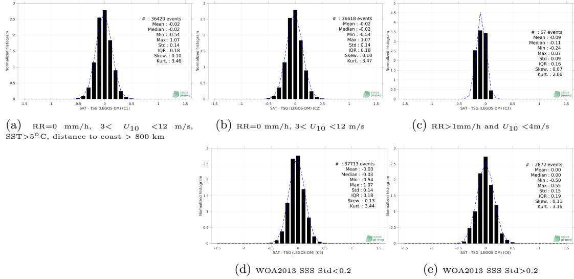
Figure 13: Normalized histogram of \Delta\text{SSS} (Aquarius SSS L3 OR v5 - Monthly (NASA-GSFC) - TSG (LEGOS-DM)) for 5 different subdatasets corresponding to: RR=0 mm/h, 3 < U_{10} < 12 m/s, SST>5°C, distance to coast > 800 km (a), RR=0 mm/h, 3 < U_{10} < 12 m/s (b), RR>1mm/h and U_{10} < 4 m/s (c), WOA2013 SSS Std<0.2 (d), WOA2013 SSS Std>0.2 (e).
