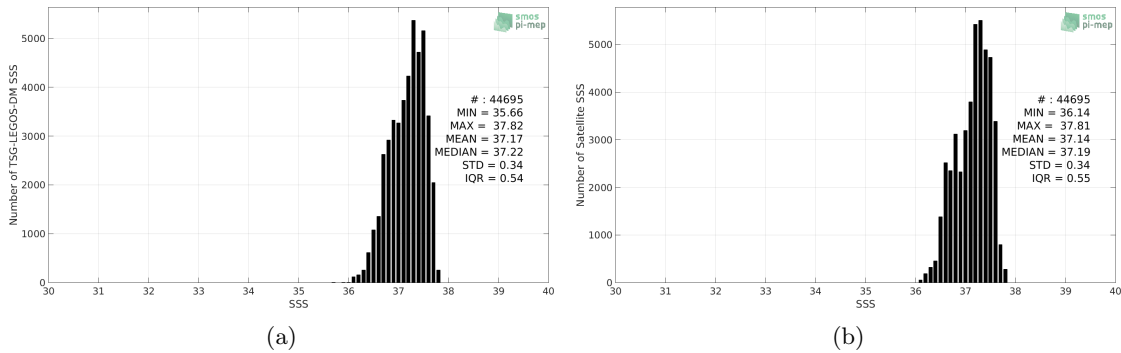
Figure 2: Histograms of SSS from TSG-LEGOS-DM (a) and Aquarius-L3-OR-V5-MONTHLY-1DEG (b) considering all match-up pairs per bins of 0.1 over the SPURS 1 Pi-MEP region and for the full satellite product period.
