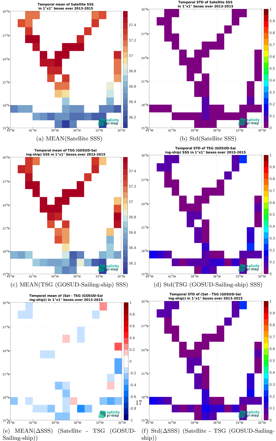
Figure 6: Temporal mean (left) and Std (right) of SSS from Aquarius SSS L3 OR v5 - Monthly (NASA-GSFC) (top), TSG (GOSUD-Sailing-ship) (middle), and of \Delta SSS (Satellite - TSG (GOSUD-Sailing-ship)). Only match-up pairs are used to generate these maps.
