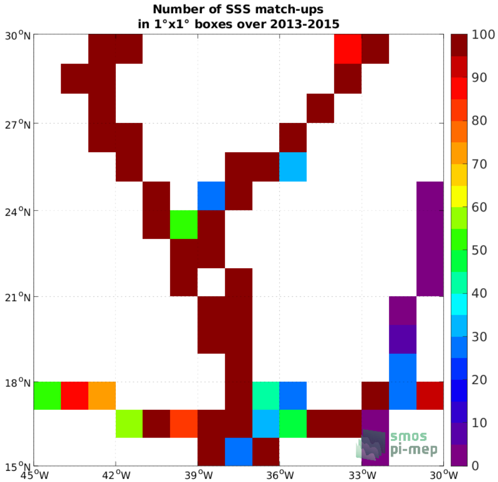
Figure 4: Number of SSS match-ups between TSG (GOSUD-Sailing-ship) SSS and the Aquarius SSS L3 OR v5 - Monthly (NASA-GSFC) SSS product for the SPURS 1 Pi-MEP region over 1°x1° boxes and for the full satellite product period.
