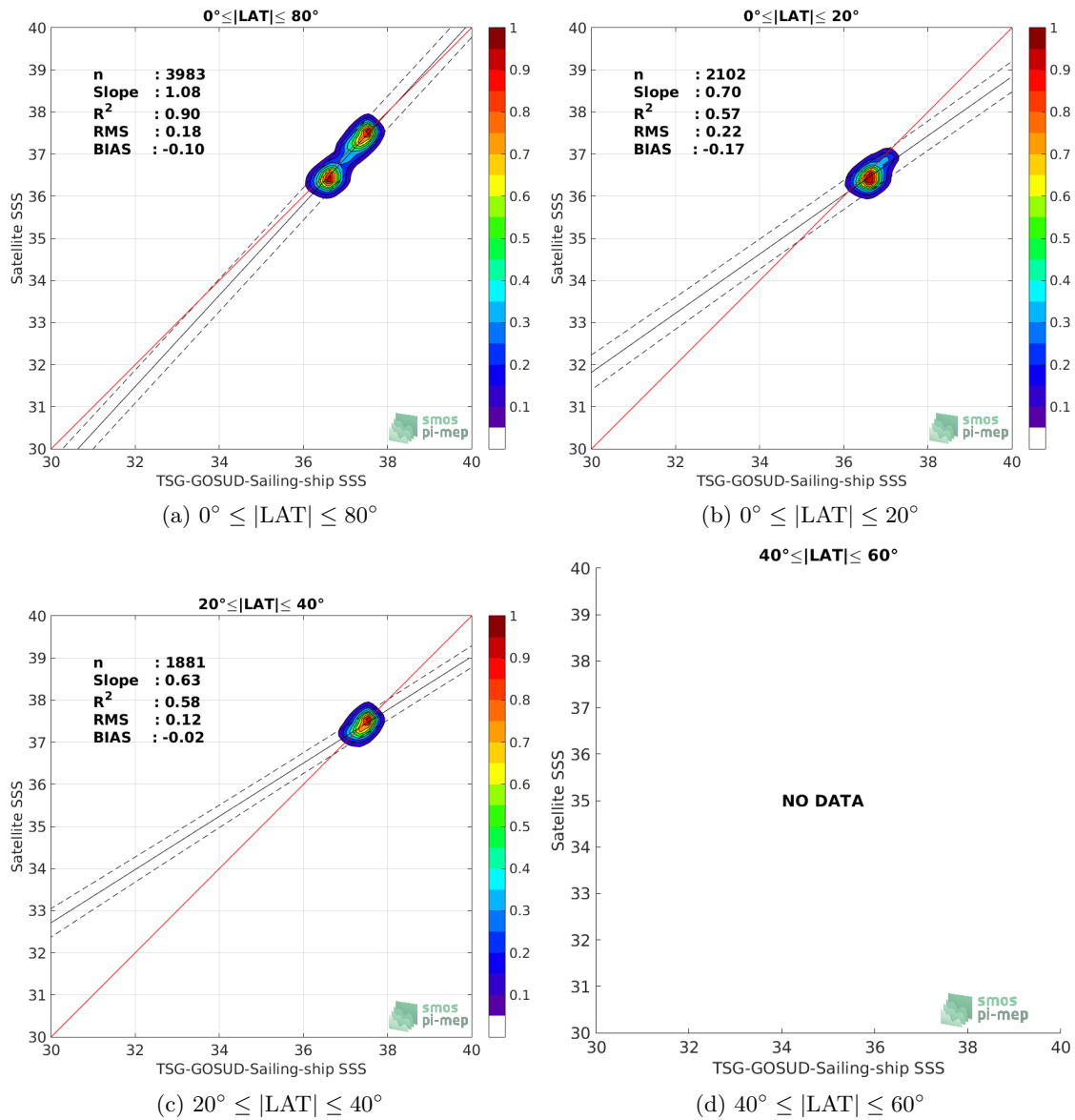
Figure 9: Contour maps of the concentration of Aquarius-L3-OR-V5-MONTHLY-1DEG SSS (y-axis) versus TSG-GOSUD-Sailing-ship SSS (x-axis) at match-up pairs for different latitude bands. For each plot, the red line shows x=y . The black thin and dashed lines indicate a linear fit through the data cloud and the \pm 95\% confidence levels, respectively. The number match-up pairs n , the slope and R^2 coefficient of the linear fit, the root mean square (RMS) and the mean bias between satellite and in situ data are indicated for each latitude band in each plots.
