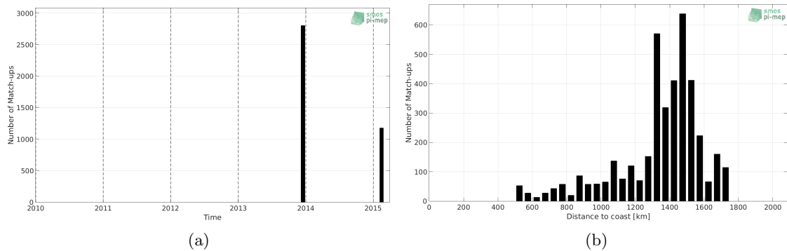
Figure 1: Number of match-ups between TSG-GOSUD-Sailing-ship and Aquarius-L3-OR-V5-MONTHLY-1DEG SSS as a function of time (a) and as function of the distance to coast (b) over the SPURS 1 Pi-MEP region and for the full satellite product period.
