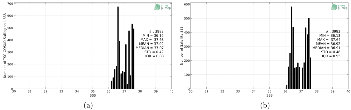
Figure 2: Histograms of SSS from TSG-GOSUD-Sailing-ship (a) and Aquarius-L3-OR-V5-MONTHLY-1DEG (b) considering all match-up pairs per bins of 0.1 over the SPURS 1 Pi-MEP region and for the full satellite product period.
