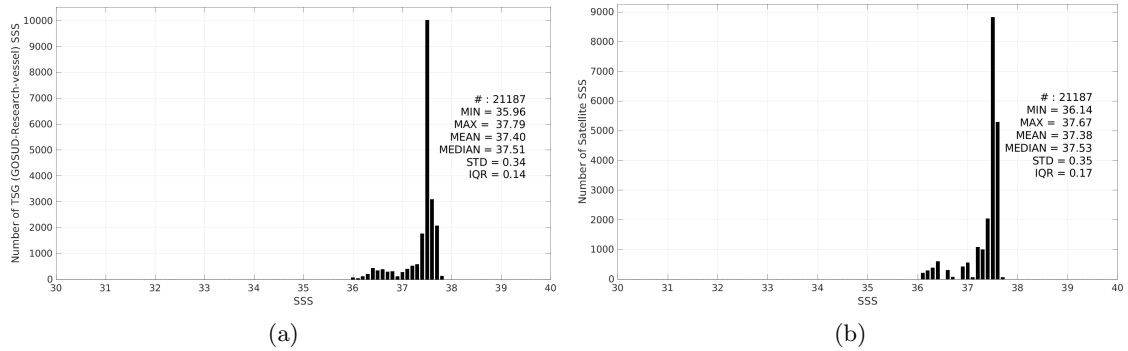
Figure 3: Histograms of SSS from TSG (GOSUD-Research-vessel) (a) and Aquarius SSS L3 OR v5 - Monthly (NASA-GSFC) (b) considering all match-up pairs per bins of 0.1 over the SPURS 1 Pi-MEP region and for the full satellite product period.
