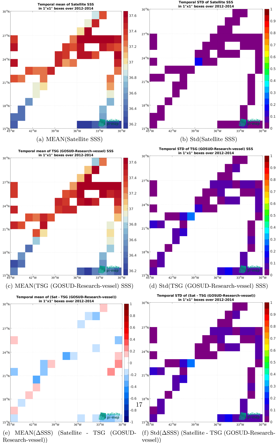
Figure 7: Temporal mean (left) and Std (right) of SSS from Aquarius SSS L3 OR v5 - Monthly (NASA-GSFC) (top), TSG (GOSUD-Research-vessel) (middle), and of \Delta SSS (Satellite - TSG (GOSUD-Research-vessel)). Only match-up pairs are used to generate these maps.
