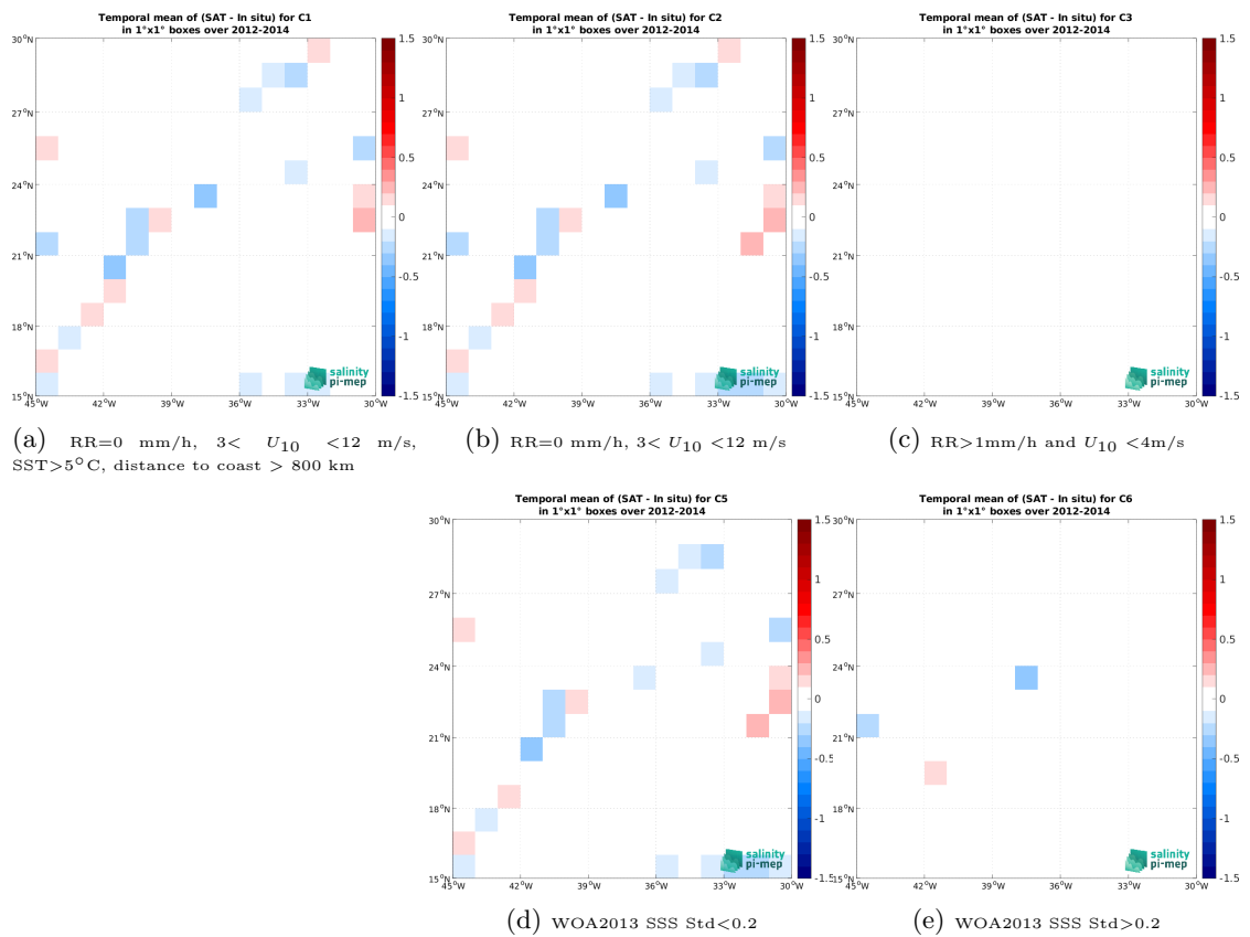
Figure 14: Temporal mean gridded over spatial boxes of size 1^\circ \times 1^\circ of \Delta SSS (Aquarius SSS L3 OR v5 - Monthly (NASA-GSFC) - TSG (GOSUD-Research-vessel)) for 5 different subdatasets corresponding to: RR=0 mm/h, 3 < U_{10} < 12 m/s, SST > 5^\circ C , distance to coast > 800 km (a), RR=0 mm/h, 3 < U_{10} < 12 m/s (b), RR > 1 mm/h and U_{10} < 4 m/s (c), WOA2013 SSS Std < 0.2 (d), WOA2013 SSS Std > 0.2 (e).
