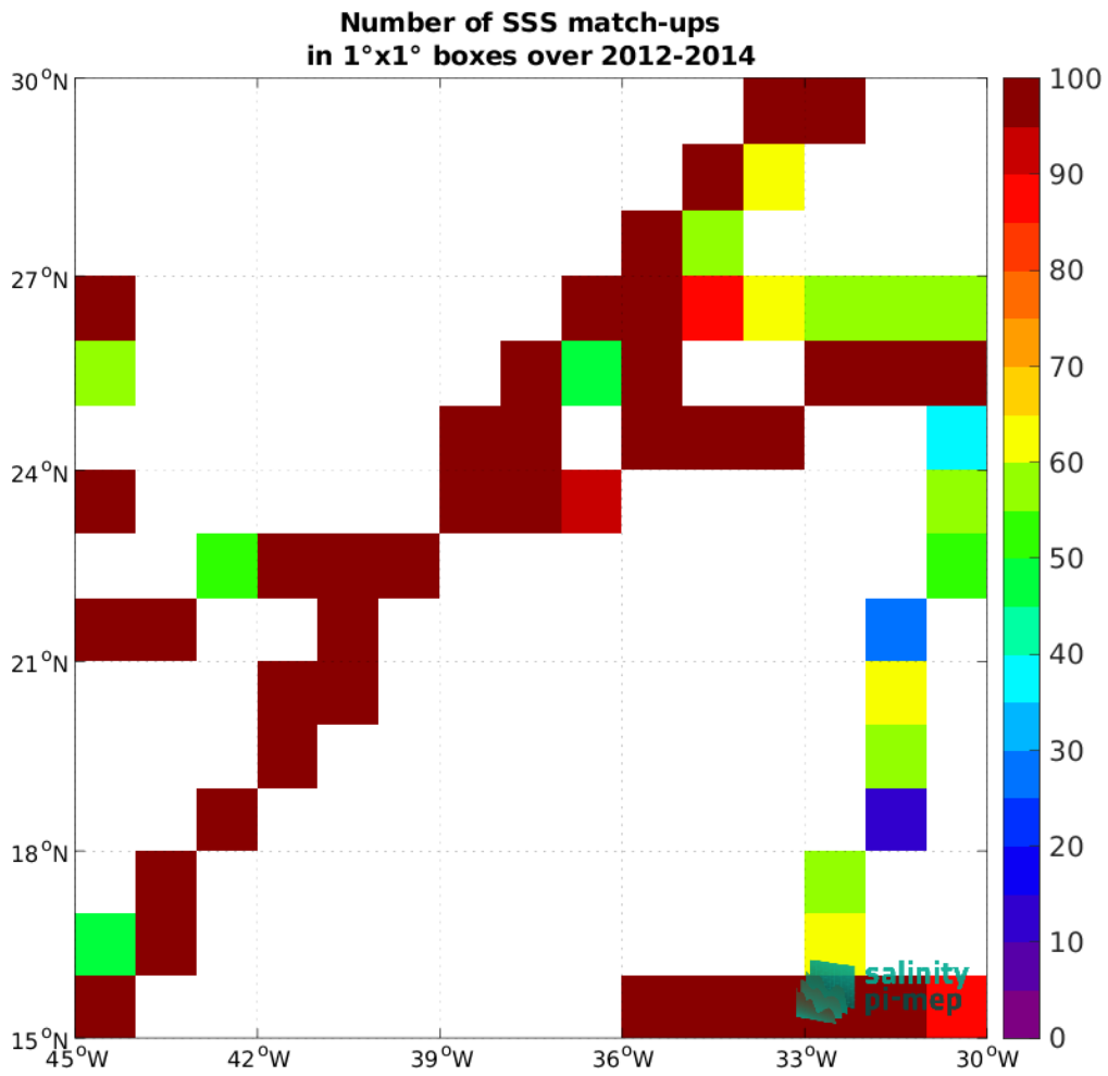
Figure 5: Number of SSS match-ups between TSG (GOSUD-Research-vessel) SSS and the Aquarius SSS L3 OR v5 - Monthly (NASA-GSFC) SSS product for the SPURS 1 Pi-MEP region over 1^\circ \times 1^\circ boxes and for the full satellite product period.
