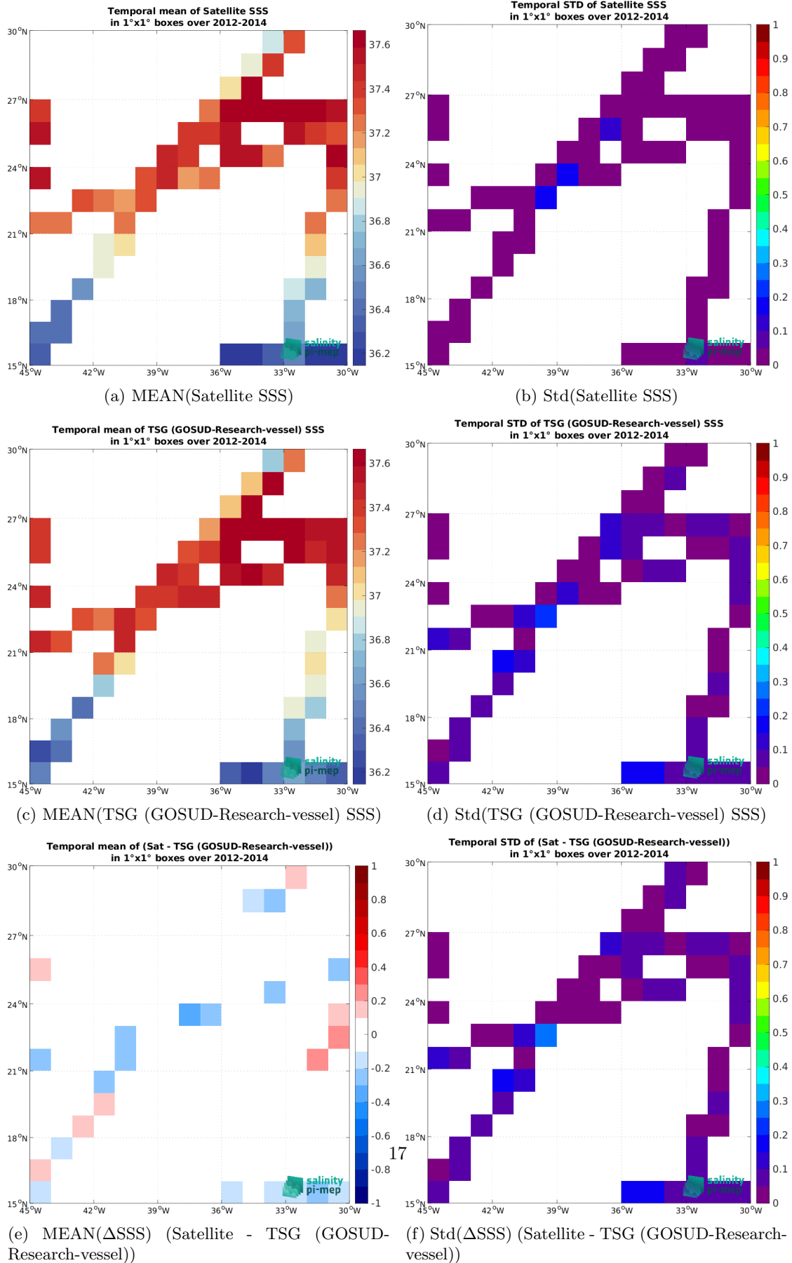
Figure 6: Temporal mean (left) and Std (right) of SSS from Aquarius SSS L3 OR v5 - Monthly (NASA-GSFC) (top), TSG (GOSUD-Research-vessel) (middle), and of \Delta SSS (Satellite - TSG (GOSUD-Research-vessel)). Only match-up pairs are used to generate these maps.
