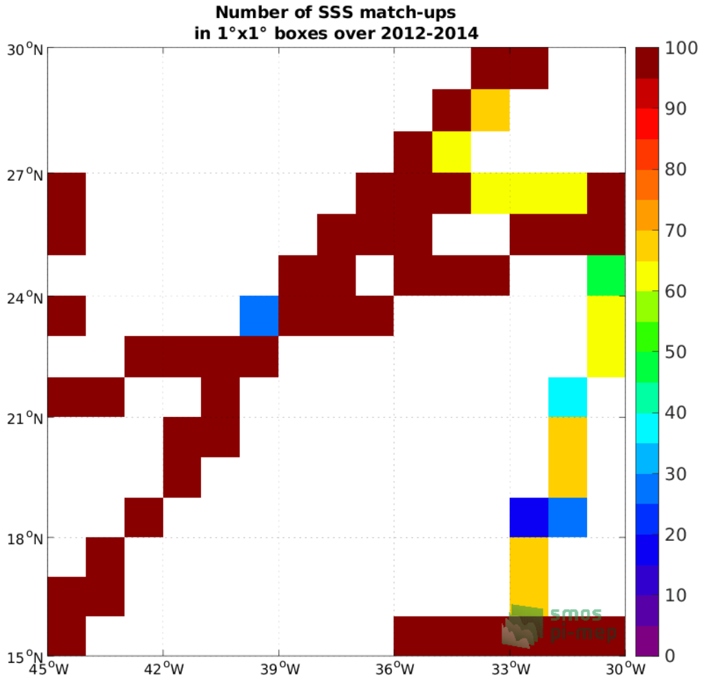
Figure 4: Number of SSS match-ups between TSG (GOSUD-Research-vessel) SSS and the Aquarius SSS L3 OR v5 - Monthly (NASA-GSFC) SSS product for the SPURS 1 Pi-MEP region over 1^\circ \times 1^\circ boxes and for the full satellite product period.
