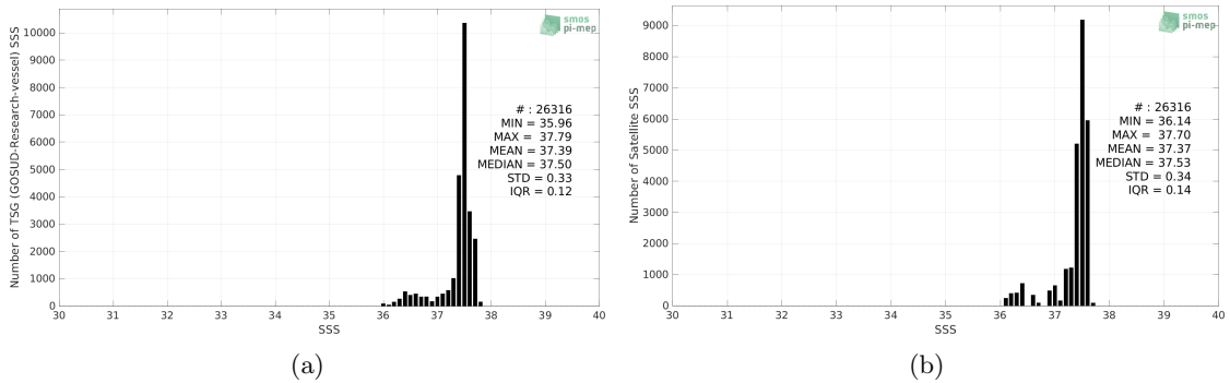
Figure 2: Histograms of SSS from TSG (GOSUD-Research-vessel) (a) and Aquarius SSS L3 OR v5 - Monthly (NASA-GSFC) (b) considering all match-up pairs per bins of 0.1 over the SPURS 1 Pi-MEP region and for the full satellite product period.
