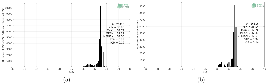
Figure 2: Histograms of SSS from TSG-GOSUD-Research-vessel (a) and Aquarius-L3-OR-V5-MONTHLY-1DEG (b) considering all match-up pairs per bins of 0.1 over the SPURS 1 Pi-MEP region and for the full satellite product period.
