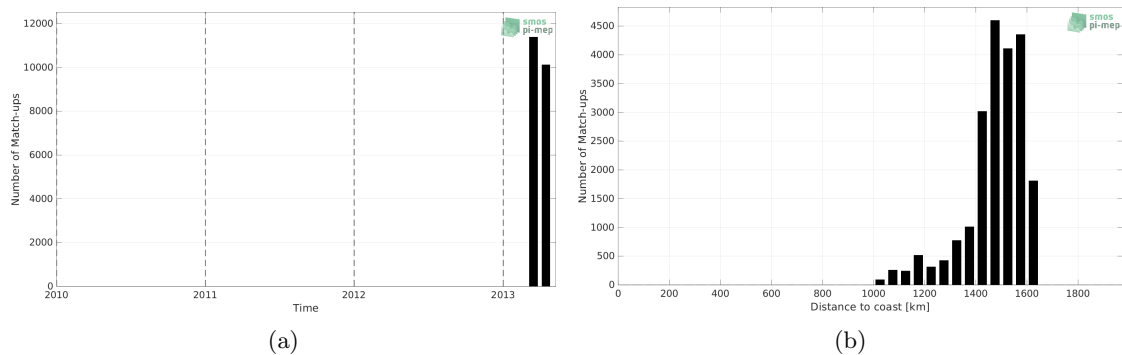
Figure 1: Number of match-ups between TSG (CSIC-UTM) and Aquarius SSS L3 OR v5 - Monthly (NASA-GSFC) SSS as a function of time (a) and as function of the distance to coast (b) over the SPURS 1 Pi-MEP region and for the full satellite product period.
