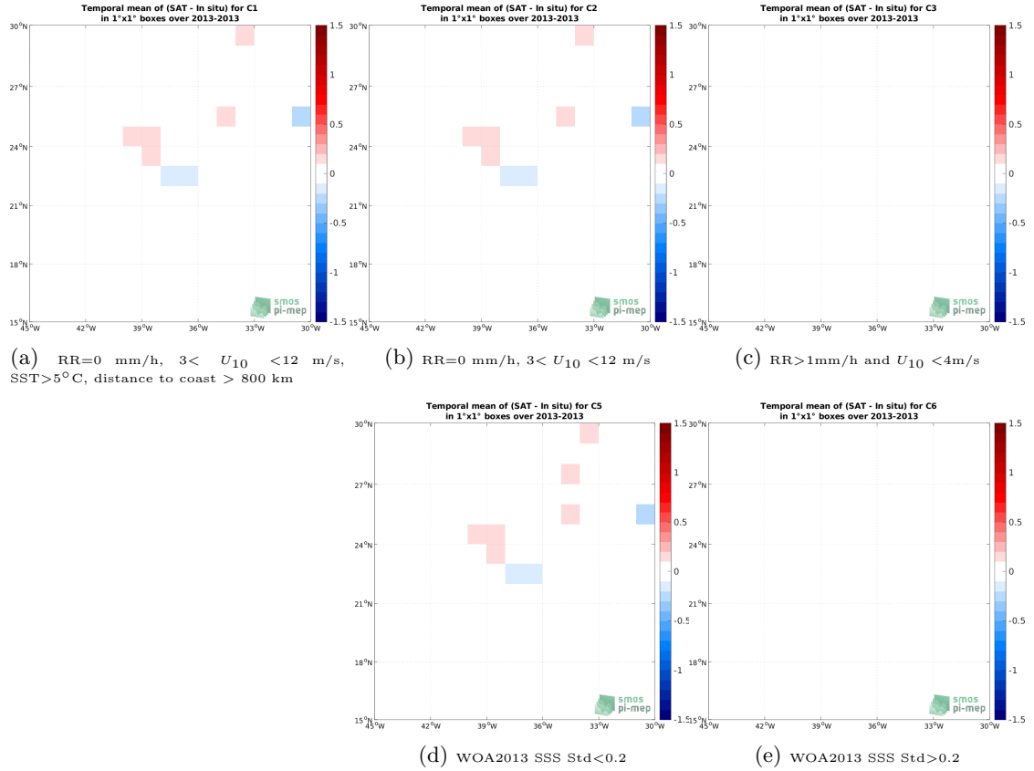
Figure 12: Temporal mean gridded over spatial boxes of size 1^{\circ}\times 1^{\circ} of \Delta\text{SSS} (Aquarius SSS L3 OR v5 - Monthly (NASA-GSFC) - TSG (CSIC-UTM)) for 5 different subdatasets corresponding to:RR=0 mm/h, 3 < U_{10} < 12 m/s, SST >5^{\circ}\text{C} , distance to coast > 800 km (a), RR=0 mm/h, 3 < U_{10} < 12 m/s (b), RR >1 mm/h and U_{10} < 4 m/s (c), WOA2013 SSS Std <0.2 (d), WOA2013 SSS Std >0.2 (e).
