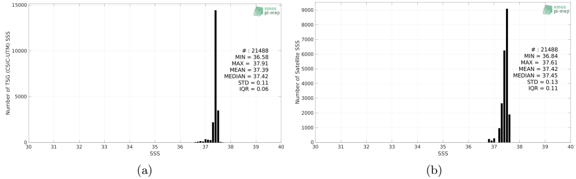
Figure 2: Histograms of SSS from TSG (CSIC-UTM) (a) and Aquarius SSS L3 OR v5 - Monthly (NASA-GSFC) (b) considering all match-up pairs per bins of 0.1 over the SPURS 1 Pi-MEP region and for the full satellite product period.
