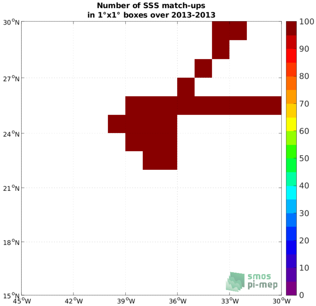
Figure 4: Number of SSS match-ups between TSG (CSIC-UTM) SSS and the Aquarius SSS L3 OR v5 - Monthly (NASA-GSFC) SSS product for the SPURS 1 Pi-MEP region over 1°x1° boxes and for the full satellite product period.
