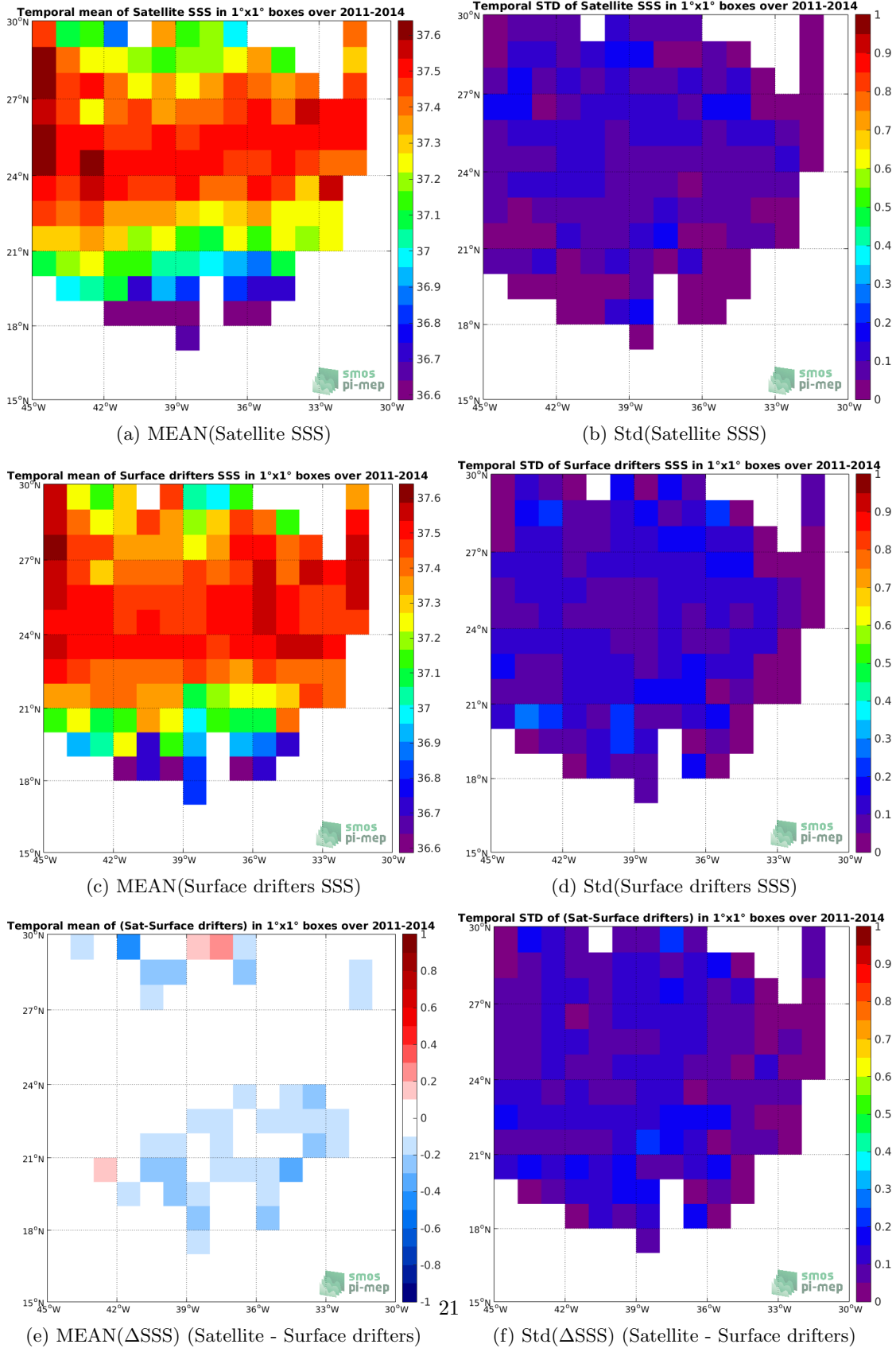
Figure 5: Temporal mean (left) and Std (right) of SSS from Aquarius-L3-OR-V5-MONTHLY-1DEG (top), Surface drifters (middle), and of \Delta SSS (Satellite - Surface drifters). Only match-up pairs are used to generate these maps.
