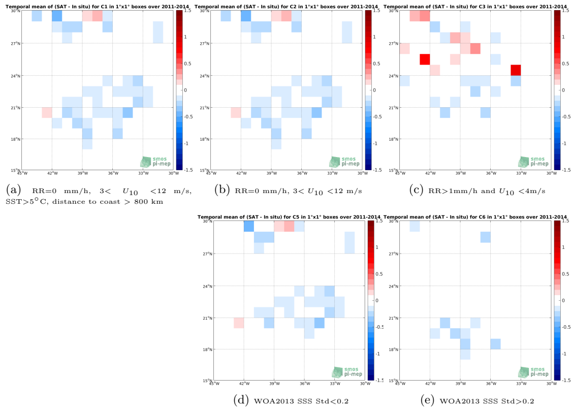
Figure 11: Temporal mean gridded over spatial boxes of size 1^\circ \times 1^\circ of \Delta SSS (Aquarius-L3-OR-V5-MONTHLY-1DEG - Surface drifters) for 5 different subdatasets corresponding to:RR=0 mm/h, 3 < U_{10} < 12 m/s, SST >5^\circ C, distance to coast > 800 km (a), RR=0 mm/h, 3 < U_{10} < 12 m/s (b), RR >1 mm/h and U_{10} < 4 m/s (c), WOA2013 SSS Std <0.2 (d), WOA2013 SSS Std >0.2 (e).
