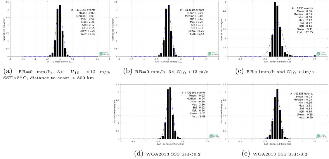
Figure 12: Normalized histogram of \Delta SSS (Aquarius-L3-OR-V5-MONTHLY-1DEG - Surface drifters) for 5 different subdatasets corresponding to: RR=0 mm/h, 3 < U_{10} < 12 m/s, SST>5°C, distance to coast > 800 km (a), RR=0 mm/h, 3 < U_{10} < 12 m/s (b), RR>1mm/h and U_{10} < 4 m/s (c), WOA2013 SSS Std<0.2 (d), WOA2013 SSS Std>0.2 (e).
