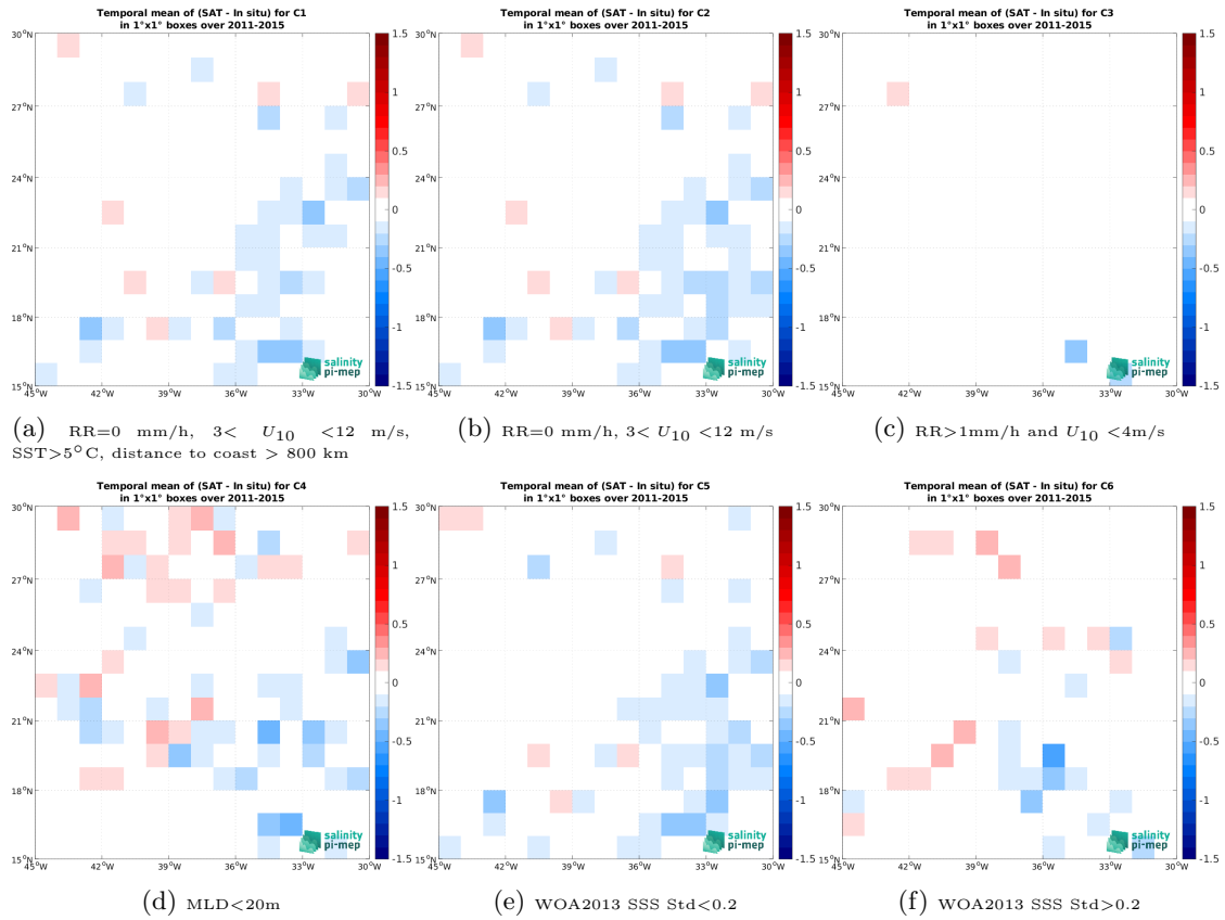
Figure 14: Temporal mean gridded over spatial boxes of size 1^\circ \times 1^\circ of \Delta\text{SSS} (Aquarius SSS L3 OR v5 - Monthly (NASA-GSFC) - Argo) for 6 different subdatasets corresponding to:RR=0 mm/h, 3 < U_{10} < 12 m/s, SST>5°C, distance to coast > 800 km (a), RR=0 mm/h, 3 < U_{10} < 12 m/s (b), RR>1mm/h and U_{10} < 4 m/s (c),MLD<20m (d),WOA2013 SSS Std<0.2 (e),WOA2013 SSS Std>0.2 (f).
