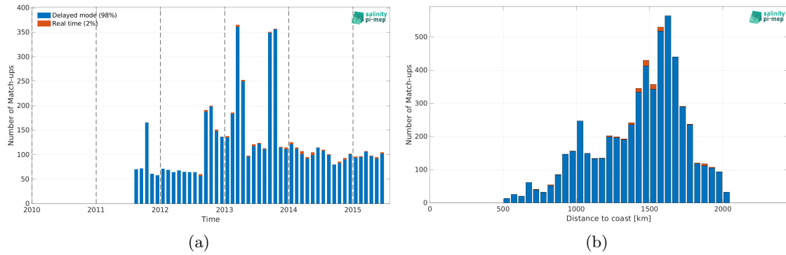
Figure 2: Number of match-ups between Argo and Aquarius SSS L3 OR v5 - Monthly (NASA-GSFC) SSS as a function of time (a) and as function of the distance to coast (b) over the SPURS 1 Pi-MEP region and for the full satellite product period.
