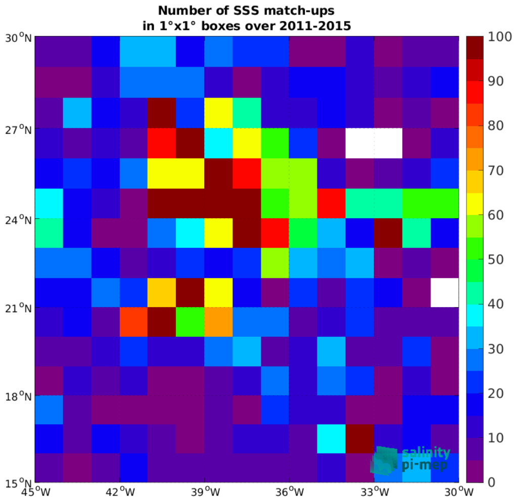
Figure 5: Number of SSS match-ups between Argo SSS and the Aquarius SSS L3 OR v5 - Monthly (NASA-GSFC) SSS product for the SPURS 1 Pi-MEP region over 1^\circ \times 1^\circ boxes and for the full satellite product period.
