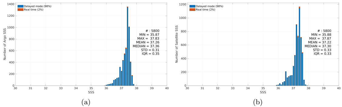
Figure 3: Histograms of SSS from Argo (a) and Aquarius SSS L3 OR v5 - Monthly (NASA-GSFC) (b) considering all match-up pairs per bins of 0.1 over the SPURS 1 Pi-MEP region and for the full satellite product period.
