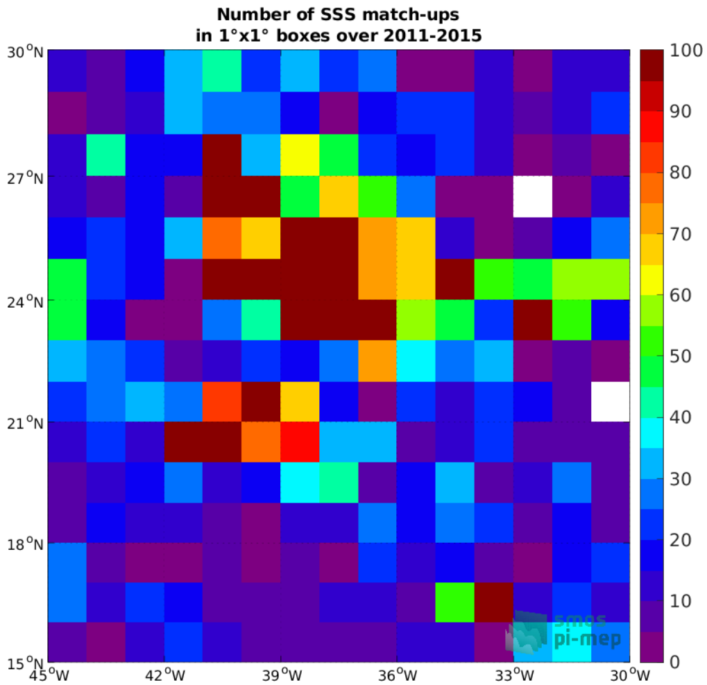
Figure 4: Number of SSS match-ups between Argo SSS and the Aquarius SSS L3 OR v5 - Monthly (NASA-GSFC) SSS product for the SPURS 1 Pi-MEP region over 1°×1° boxes and for the full satellite product period.
