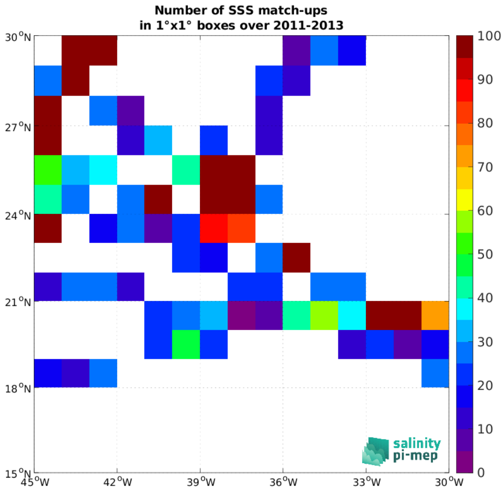
Figure 5: Number of SSS match-ups between TSG (SAMOS) SSS and the Aquarius SSS L3 OR v5 - Monthly - Rain mask (NASA-GSFC) SSS product for the SPURS 1 Pi-MEP region over 1^\circ \times 1^\circ boxes and for the full satellite product period.
