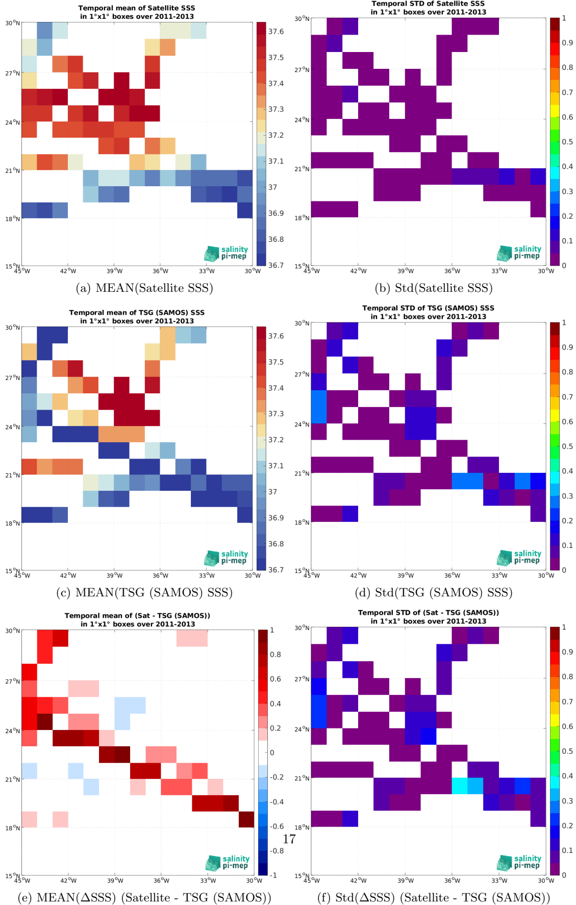
Figure 7: Temporal mean (left) and Std (right) of SSS from Aquarius SSS L3 OR v5 - Monthly - Rain mask (NASA-GSFC) (top), TSG (SAMOS) (middle), and of \Delta SSS (Satellite - TSG (SAMOS)). Only match-up pairs are used to generate these maps.
