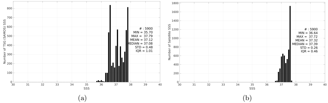
Figure 3: Histograms of SSS from TSG (SAMOS) (a) and Aquarius SSS L3 OR v5 - Monthly - Rain mask (NASA-GSFC) (b) considering all match-up pairs per bins of 0.1 over the SPURS 1 Pi-MEP region and for the full satellite product period.
