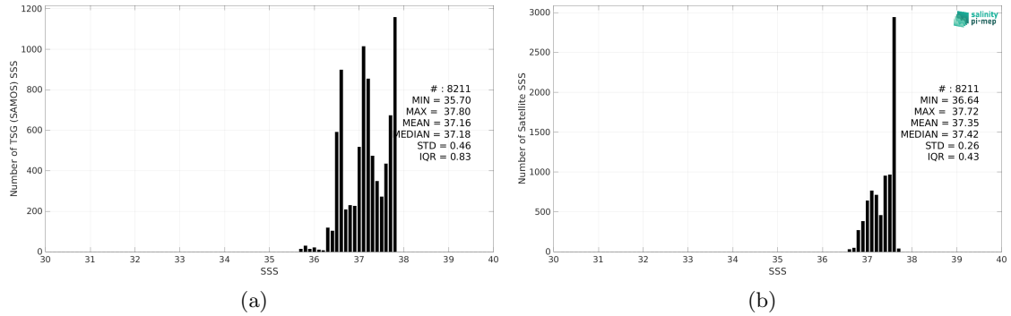
Figure 2: Histograms of SSS from TSG (SAMOS) (a) and Aquarius SSS L3 OR v5 - Monthly - Rain mask (NASA-GSFC) (b) considering all match-up pairs per bins of 0.1 over the SPURS 1 Pi-MEP region and for the full satellite product period.
