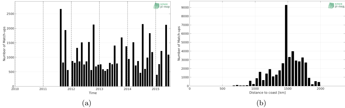
Figure 1: Number of match-ups between TSG-LEGOS-DM and Aquarius-L3-OR-V5-MONTHLY-RAIN-MASK-1DEG SSS as a function of time (a) and as function of the distance to coast (b) over the SPURS 1 Pi-MEP region and for the full satellite product period.
