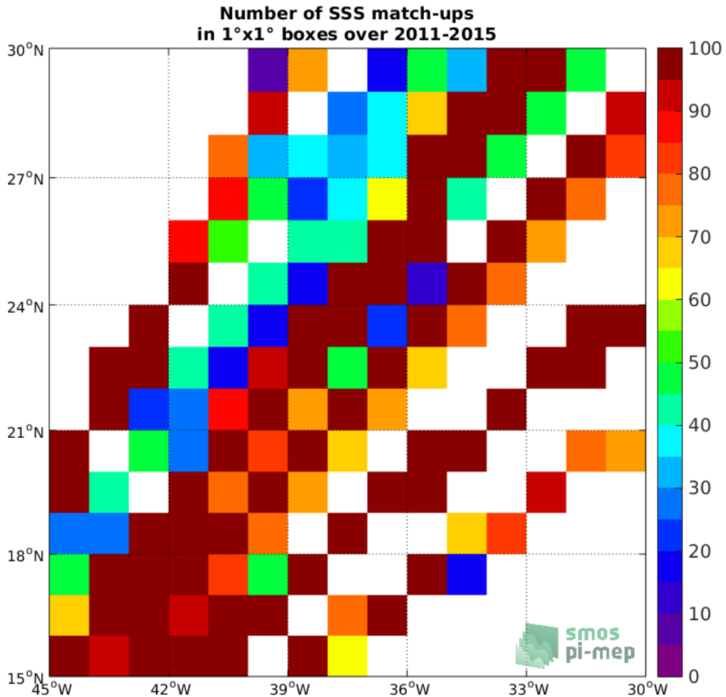
Figure 4: Number of SSS match-ups between TSG-LEGOS-DM SSS and the Aquarius-L3-OR-V5-MONTHLY-RAIN-MASK-1DEG SSS product for the SPURS 1 Pi-MEP region over 1°x1° boxes and for the full satellite product period.
