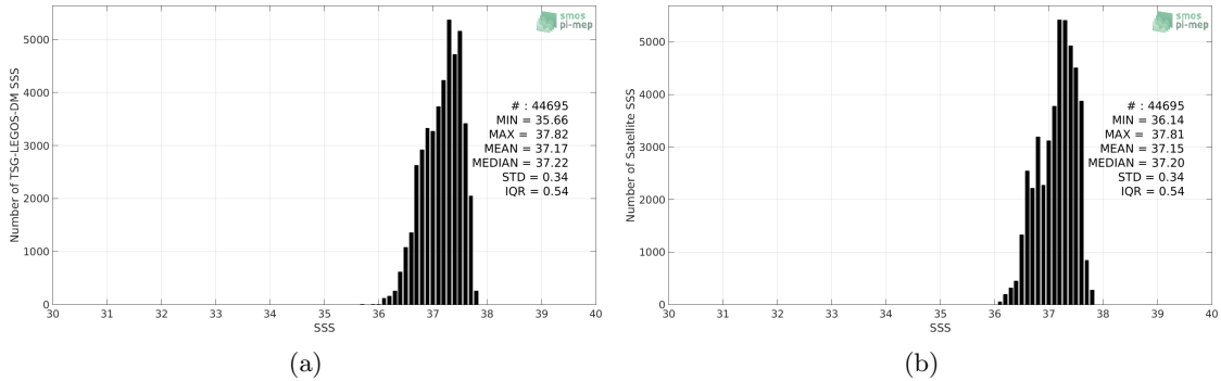
Figure 2: Histograms of SSS from TSG-LEGOS-DM (a) and Aquarius-L3-OR-V5-MONTHLY-RAIN-MASK-1DEG (b) considering all match-up pairs per bins of 0.1 over the SPURS 1 Pi-MEP region and for the full satellite product period.
