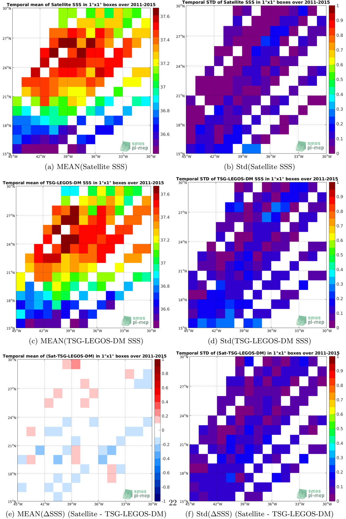
Figure 6: Temporal mean (left) and Std (right) of SSS from Aquarius-L3-OR-V5-MONTHLY-RAIN-MASK-1DEG (top), TSG-LEGOS-DM (middle), and of \Delta SSS (Satellite - TSG-LEGOS-DM). Only match-up pairs are used to generate these maps.
