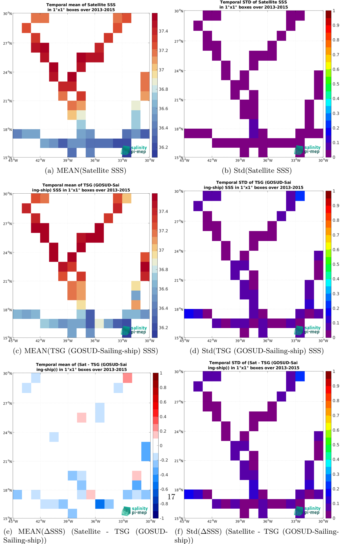
Figure 7: Temporal mean (left) and Std (right) of SSS from Aquarius SSS L3 OR v5 - Monthly - Rain mask (NASA-GSFC) (top), TSG (GOSUD-Sailing-ship) (middle), and of \Delta SSS (Satellite - TSG (GOSUD-Sailing-ship)). Only match-up pairs are used to generate these maps.
