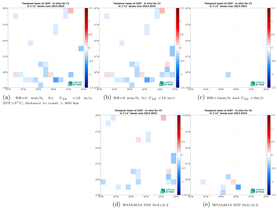
Figure 14: Temporal mean gridded over spatial boxes of size 1^\circ \times 1^\circ of \Delta SSS (Aquarius SSS L3 OR v5 - Monthly - Rain mask (NASA-GSFC) - TSG (GOSUD-Sailing-ship)) for 5 different subdatasets corresponding to: RR=0 mm/h, 3 < U_{10} < 12 m/s, SST > 5^\circ C , distance to coast > 800 km (a), RR=0 mm/h, 3 < U_{10} < 12 m/s (b), RR > 1 mm/h and U_{10} < 4 m/s (c), WOA2013 SSS Std < 0.2 (d), WOA2013 SSS Std > 0.2 (e).
