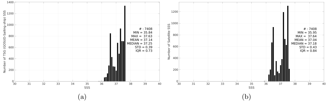
Figure 3: Histograms of SSS from TSG (GOSUD-Sailing-ship) (a) and Aquarius SSS L3 OR v5 - Monthly - Rain mask (NASA-GSFC) (b) considering all match-up pairs per bins of 0.1 over the SPURS 1 Pi-MEP region and for the full satellite product period.
