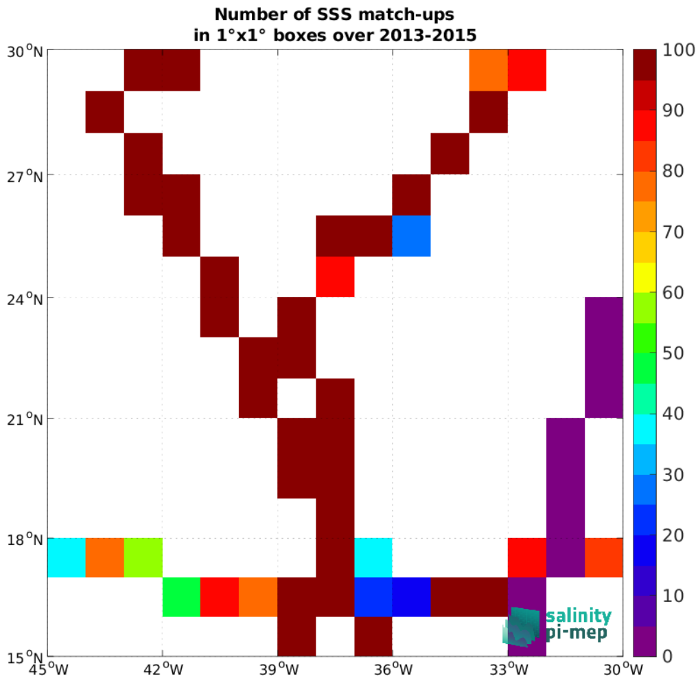
Figure 5: Number of SSS match-ups between TSG (GOSUD-Sailing-ship) SSS and the Aquarius SSS L3 OR v5 - Monthly - Rain mask (NASA-GSFC) SSS product for the SPURS 1 Pi-MEP region over 1^\circ \times 1^\circ boxes and for the full satellite product period.
