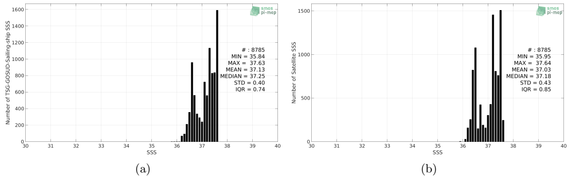
Figure 2: Histograms of SSS from TSG-GOSUD-Sailing-ship (a) and Aquarius-L3-OR-V5-MONTHLY-RAIN-MASK-1DEG (b) considering all match-up pairs per bins of 0.1 over the SPURS 1 Pi-MEP region and for the full satellite product period.
