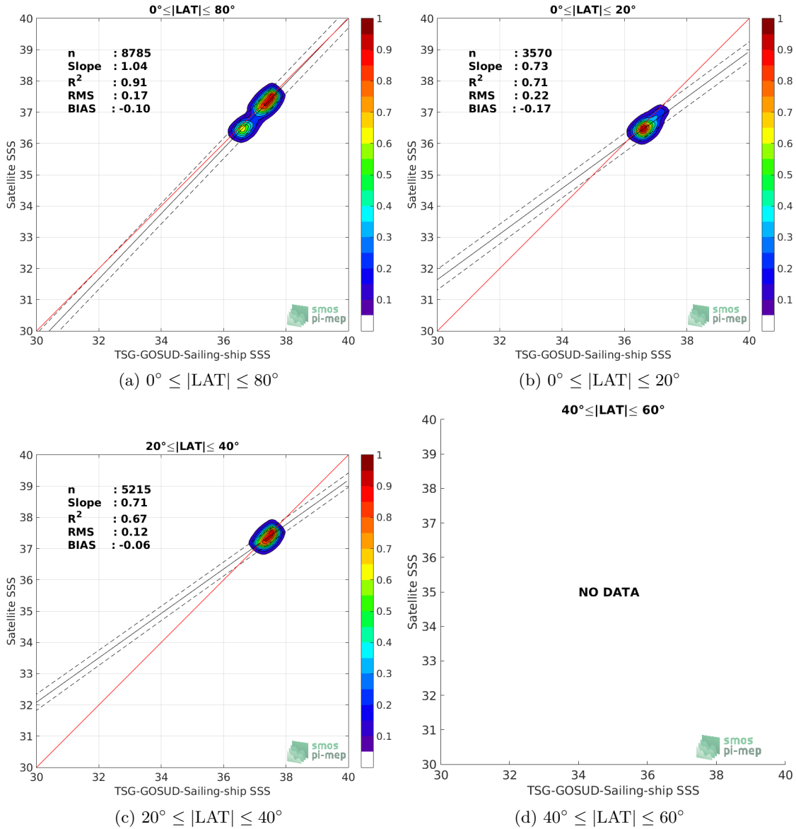
Figure 9: Contour maps of the concentration of Aquarius-L3-OR-V5-MONTHLY-RAIN-MASK-1DEG SSS (y-axis) versus TSG-GOSUD-Sailing-ship SSS (x-axis) at match-up pairs for different latitude bands. For each plot, the red line shows x=y . The black thin and dashed lines indicate a linear fit through the data cloud and the \pm 95\% confidence levels, respectively. The number match-up pairs n , the slope and R^2 coefficient of the linear fit, the root mean square (RMS) and the mean bias between satellite and in situ data are indicated for each latitude band in each plots.
