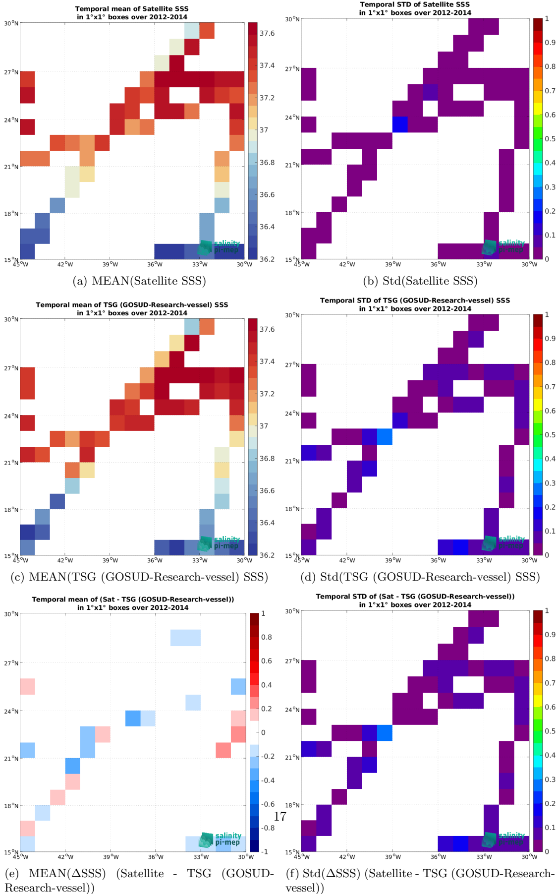
Figure 7: Temporal mean (left) and Std (right) of SSS from Aquarius SSS L3 OR v5 - Monthly - Rain mask (NASA-GSFC) (top), TSG (GOSUD-Research-vessel) (middle), and of \Delta SSS (Satellite - TSG (GOSUD-Research-vessel)). Only match-up pairs are used to generate these maps.
