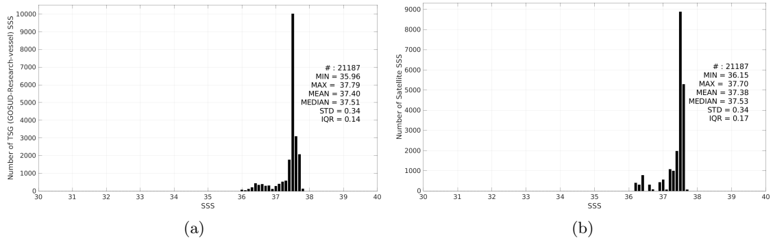
Figure 3: Histograms of SSS from TSG (GOSUD-Research-vessel) (a) and Aquarius SSS L3 OR v5 - Monthly - Rain mask (NASA-GSFC) (b) considering all match-up pairs per bins of 0.1 over the SPURS 1 Pi-MEP region and for the full satellite product period.
