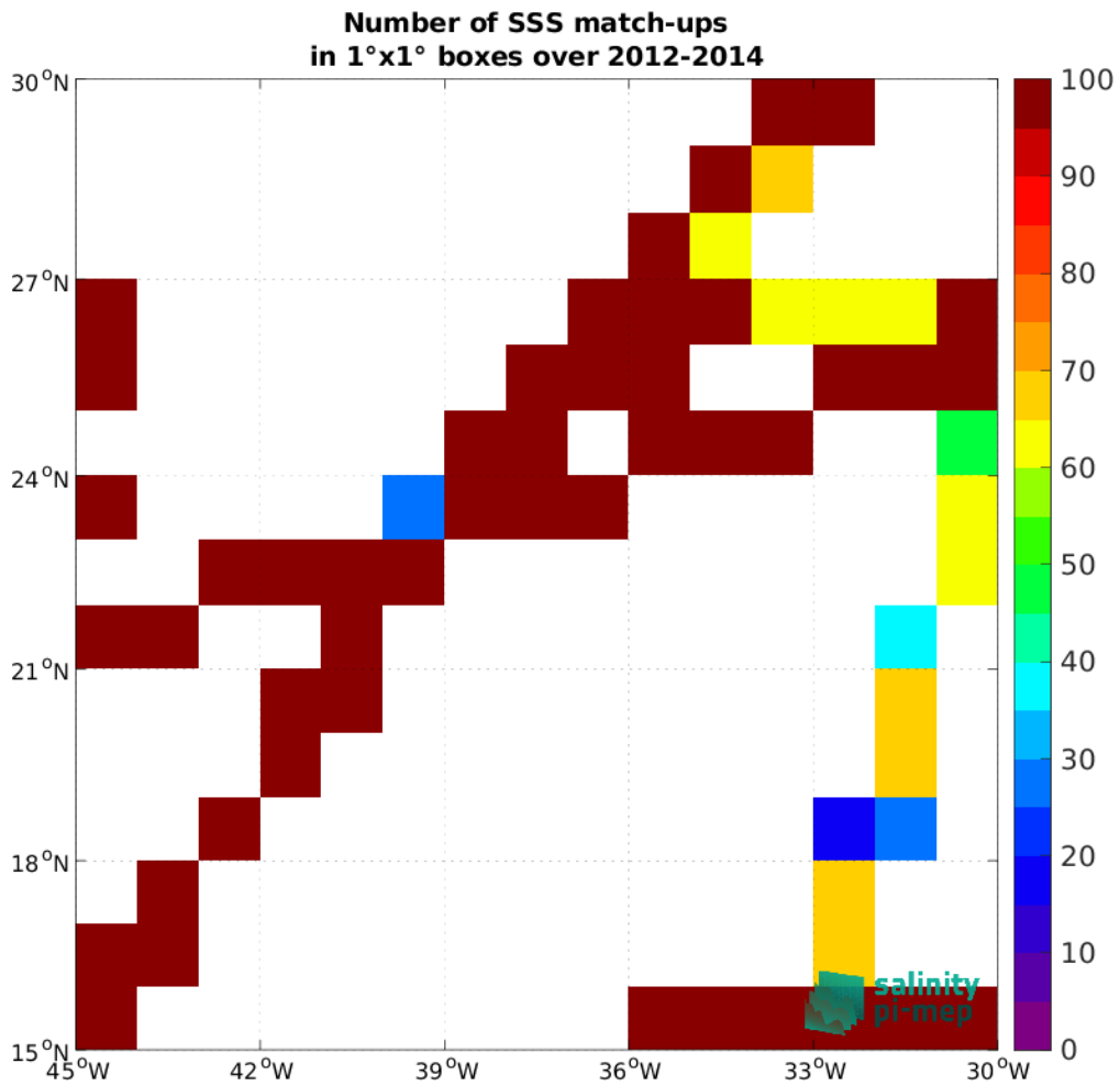
Figure 4: Number of SSS match-ups between TSG (GOSUD-Research-vessel) SSS and the Aquarius SSS L3 OR v5 - Monthly - Rain mask (NASA-GSFC) SSS product for the SPURS 1 Pi-MEP region over 1°x1° boxes and for the full satellite product period.
