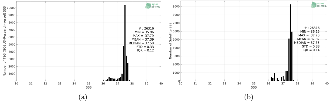
Figure 2: Histograms of SSS from TSG (GOSUD-Research-vessel) (a) and Aquarius SSS L3 OR v5 - Monthly - Rain mask (NASA-GSFC) (b) considering all match-up pairs per bins of 0.1 over the SPURS 1 Pi-MEP region and for the full satellite product period.
