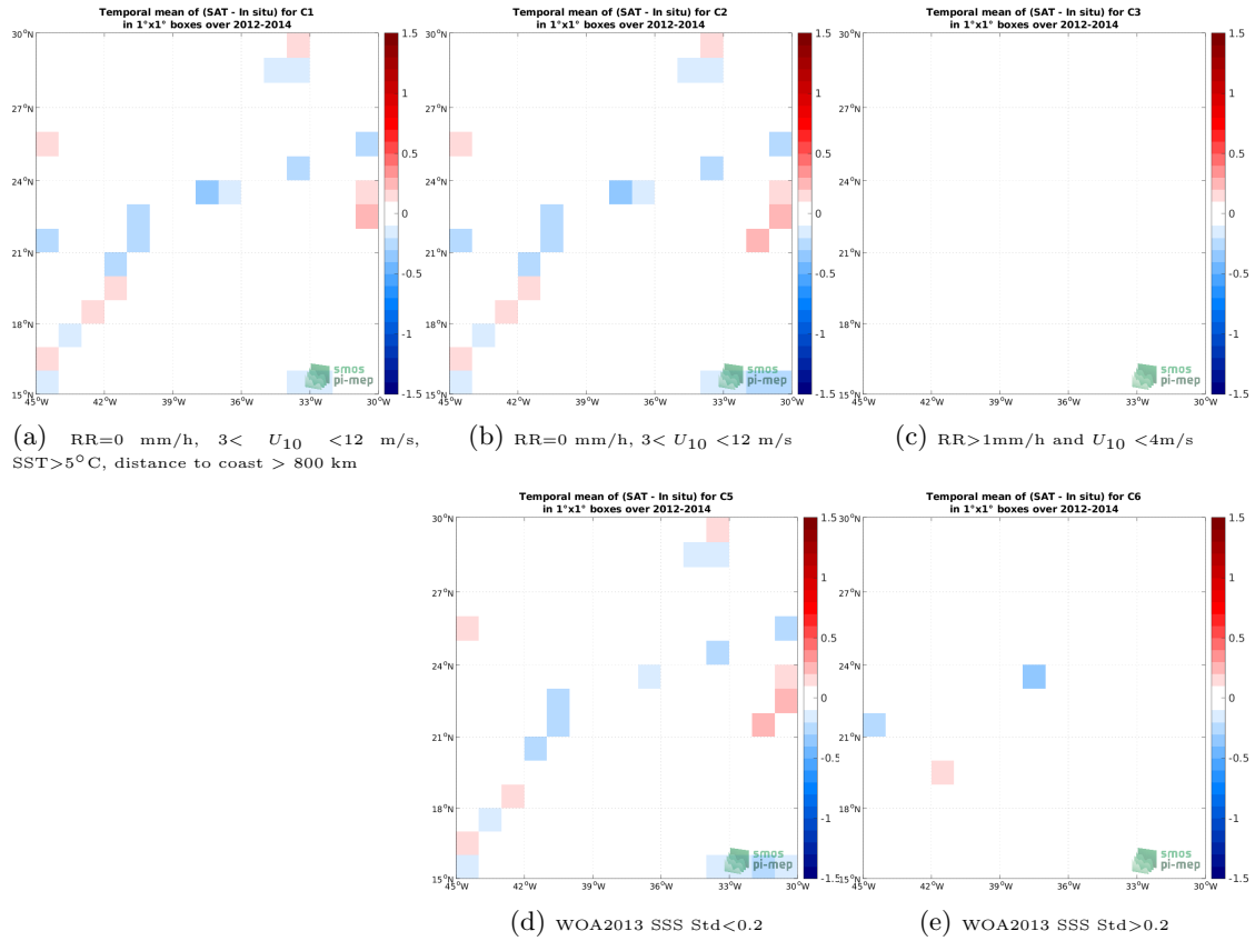
Figure 12: Temporal mean gridded over spatial boxes of size 1^\circ \times 1^\circ of \Delta SSS (Aquarius SSS L3 OR v5 - Monthly - Rain mask (NASA-GSFC) - TSG (GOSUD-Research-vessel)) for 5 different subdatasets corresponding to: RR=0 mm/h, 3 < U_{10} < 12 m/s, SST > 5°C, distance to coast > 800 km (a), RR=0 mm/h, 3 < U_{10} < 12 m/s (b), RR > 1mm/h and U_{10} < 4 m/s (c), WOA2013 SSS Std < 0.2 (d), WOA2013 SSS Std > 0.2 (e).
