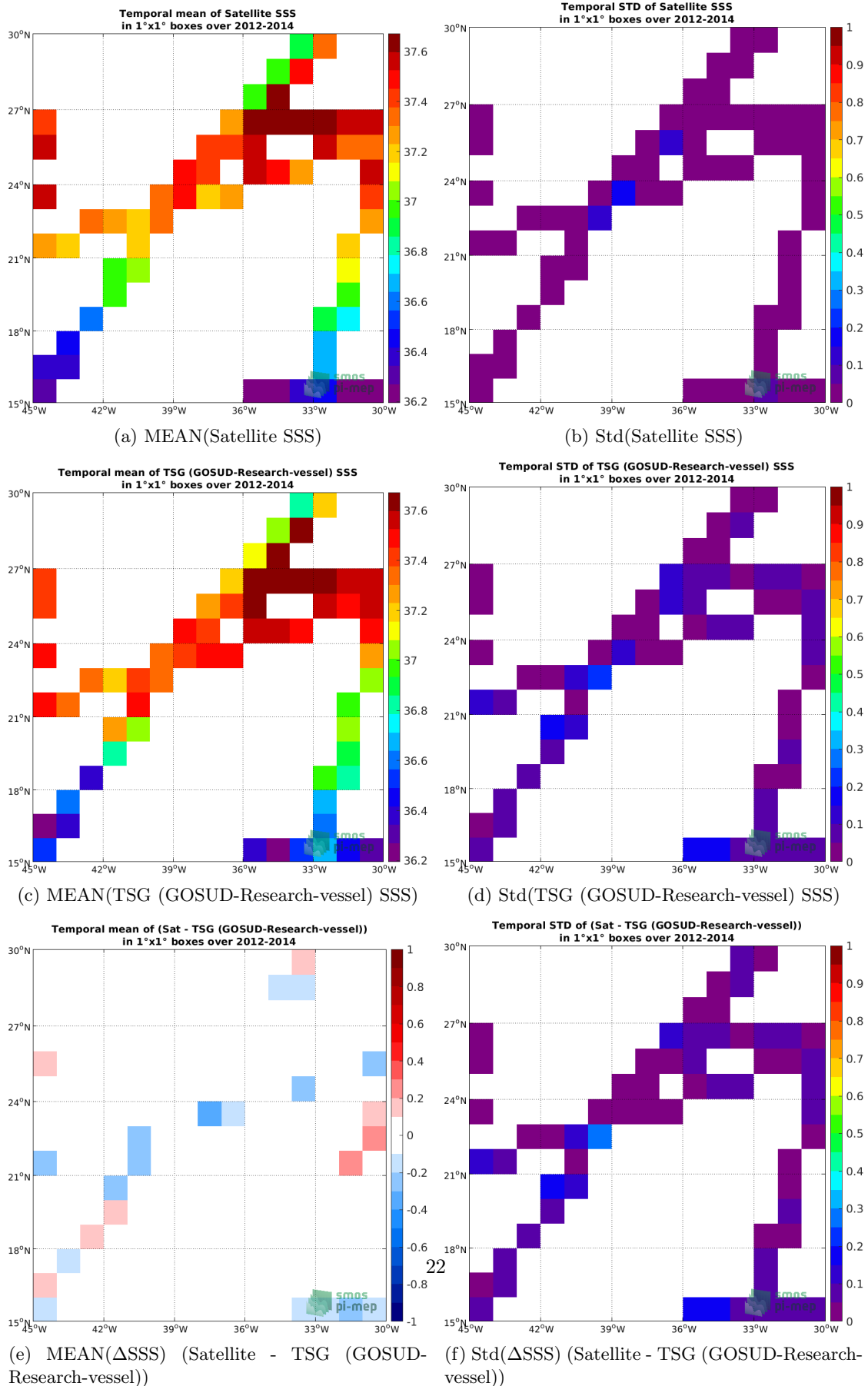
Figure 6: Temporal mean (left) and Std (right) of SSS from Aquarius SSS L3 OR v5 - Monthly - Rain mask (NASA-GSFC) (top), TSG (GOSUD-Research-vessel) (middle), and of \Delta SSS (Satellite - TSG (GOSUD-Research-vessel)). Only match-up pairs are used to generate these maps.
