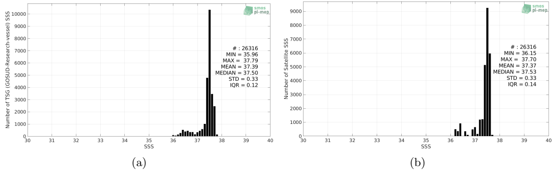
Figure 2: Histograms of SSS from TSG (GOSUD-Research-vessel) (a) and Aquarius SSS L3 OR v5 - Monthly - Rain mask (NASA-GSFC) (b) considering all match-up pairs per bins of 0.1 over the SPURS 1 Pi-MEP region and for the full satellite product period.
