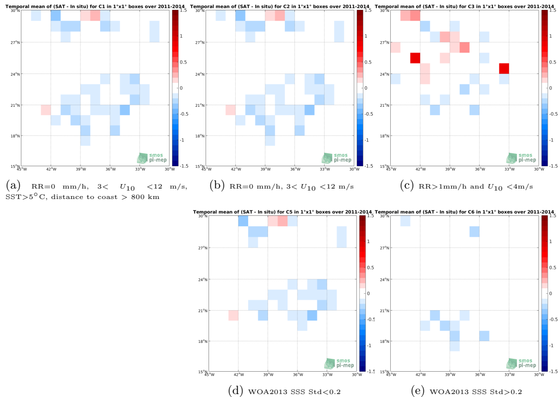
Figure 11: Temporal mean gridded over spatial boxes of size 1^\circ \times 1^\circ of \Delta SSS (Aquarius-L3-OR-V5-MONTHLY-RAIN-MASK-1DEG - Surface drifters) for 5 different subdatasets corresponding to:RR=0 mm/h, 3 < U_{10} < 12 m/s, SST >5^\circ C, distance to coast > 800 km (a), RR=0 mm/h, 3 < U_{10} < 12 m/s (b), RR >1 mm/h and U_{10} < 4 m/s (c), WOA2013 SSS Std <0.2 (d), WOA2013 SSS Std >0.2 (e).
