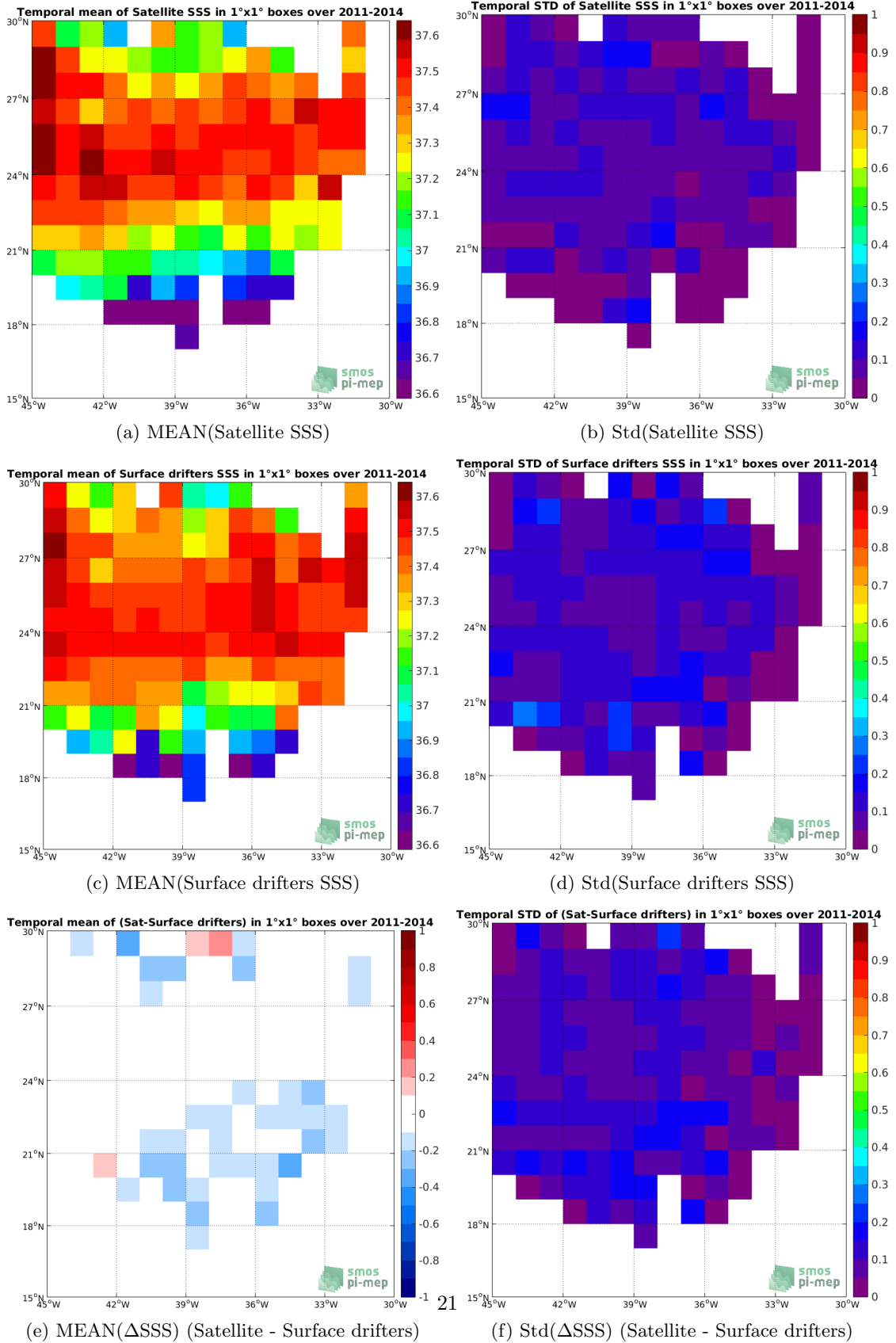
Figure 5: Temporal mean (left) and Std (right) of SSS from Aquarius-L3-OR-V5-MONTHLY-RAIN-MASK-1DEG (top), Surface drifters (middle), and of \Delta SSS (Satellite - Surface drifters). Only match-up pairs are used to generate these maps.
