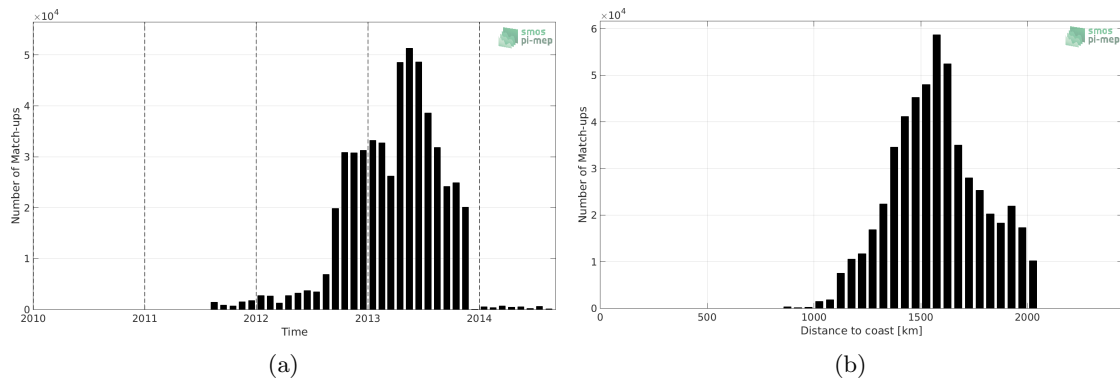
Figure 1: Number of match-ups between Surface drifters and Aquarius-L3-OR-V5-MONTHLY-RAIN-MASK-1DEG SSS as a function of time (a) and as function of the distance to coast (b) over the SPURS 1 Pi-MEP region and for the full satellite product period.
