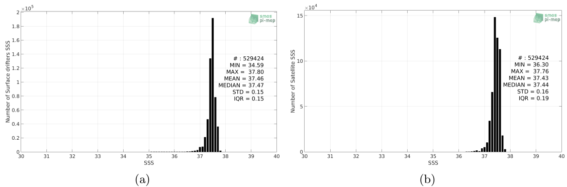
Figure 2: Histograms of SSS from Surface drifters (a) and Aquarius-L3-OR-V5-MONTHLY-RAIN-MASK-1DEG (b) considering all match-up pairs per bins of 0.1 over the SPURS 1 Pi-MEP region and for the full satellite product period.
