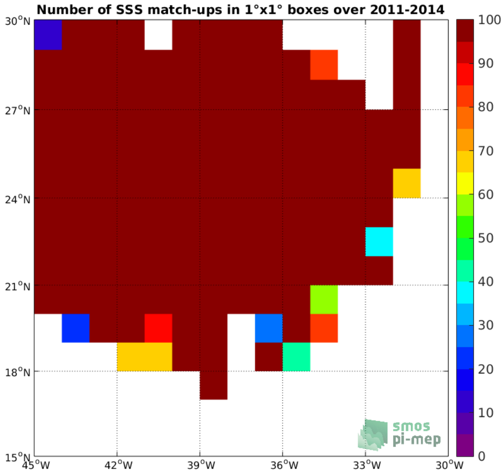
Figure 3: Number of SSS match-ups between Surface drifters SSS and the Aquarius-L3-OR-V5-MONTHLY-RAIN-MASK-1DEG SSS product for the SPURS 1 Pi-MEP region over 1°x1° boxes and for the full satellite product period.
