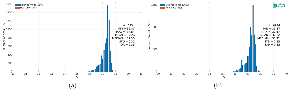
Figure 2: Histograms of SSS from Argo (a) and Aquarius SSS L3 OR v5 - Monthly - Rain mask (NASA-GSFC) (b) considering all match-up pairs per bins of 0.1 over the SPURS 1 Pi-MEP region and for the full satellite product period.
