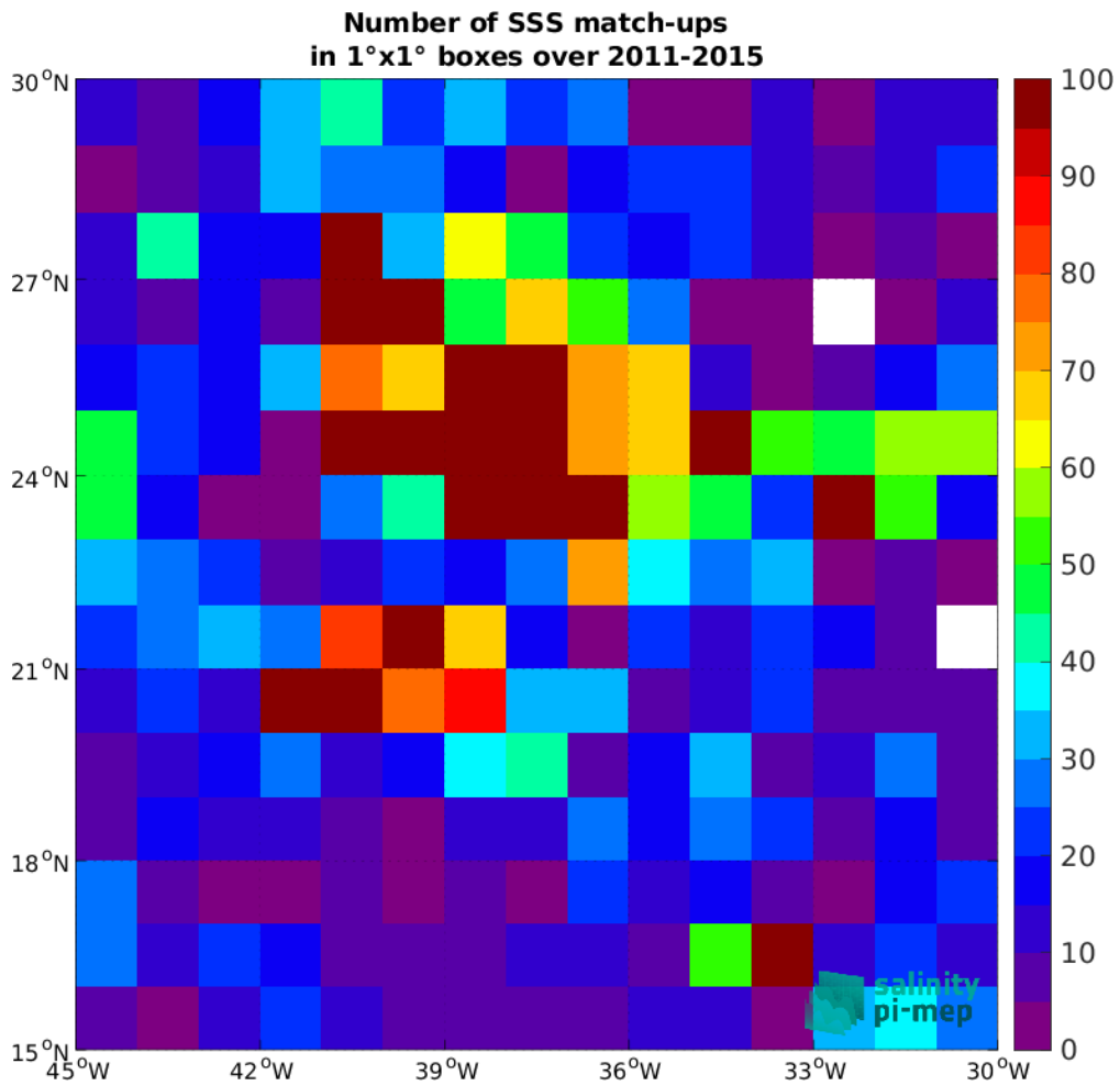
Figure 4: Number of SSS match-ups between Argo SSS and the Aquarius SSS L3 OR v5 - Monthly - Rain mask (NASA-GSFC) SSS product for the SPURS 1 Pi-MEP region over 1°x1° boxes and for the full satellite product period.
