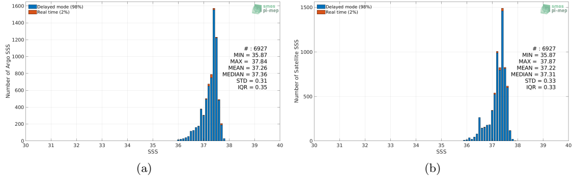
Figure 2: Histograms of SSS from Argo (a) and Aquarius SSS L3 OR v5 - Monthly - Rain mask (NASA-GSFC) (b) considering all match-up pairs per bins of 0.1 over the SPURS 1 Pi-MEP region and for the full satellite product period.
