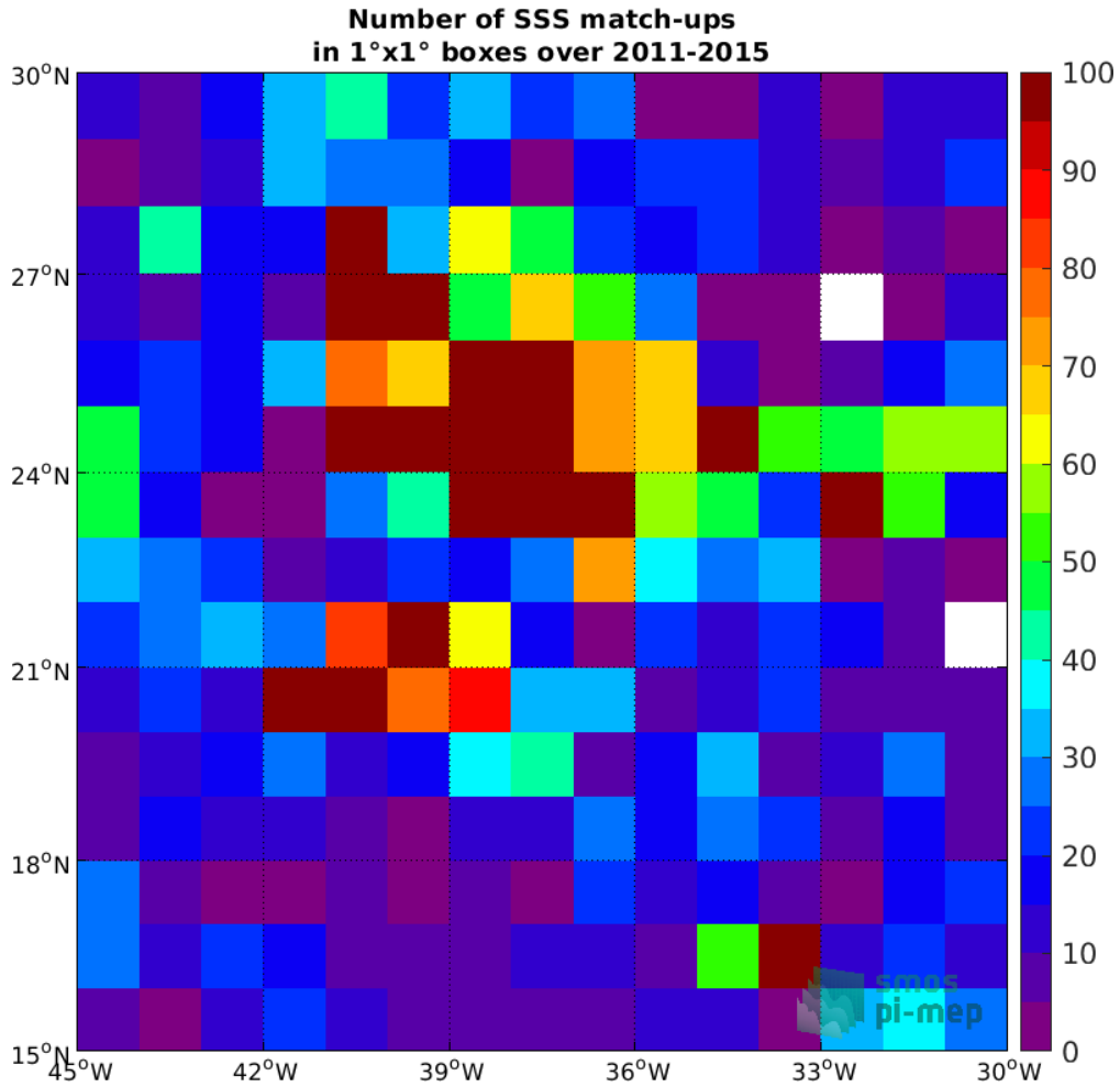
Figure 4: Number of SSS match-ups between Argo SSS and the Aquarius SSS L3 OR v5 - Monthly - Rain mask (NASA-GSFC) SSS product for the SPURS 1 Pi-MEP region over 1^\circ \times 1^\circ boxes and for the full satellite product period.
