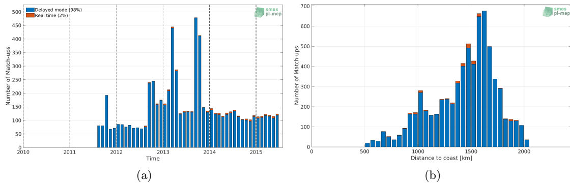
Figure 1: Number of match-ups between Argo and Aquarius SSS L3 OR v5 - Monthly - Rain mask (NASA-GSFC) SSS as a function of time (a) and as function of the distance to coast (b) over the SPURS 1 Pi-MEP region and for the full satellite product period.
