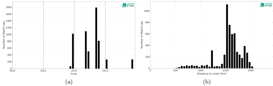
Figure 2: Number of match-ups between TSG (SAMOS) and Aquarius SSS L3 CAP v5 - 7-Day running (JPL) SSS as a function of time (a) and as function of the distance to coast (b) over the SPURS 1 Pi-MEP region and for the full satellite product period.
