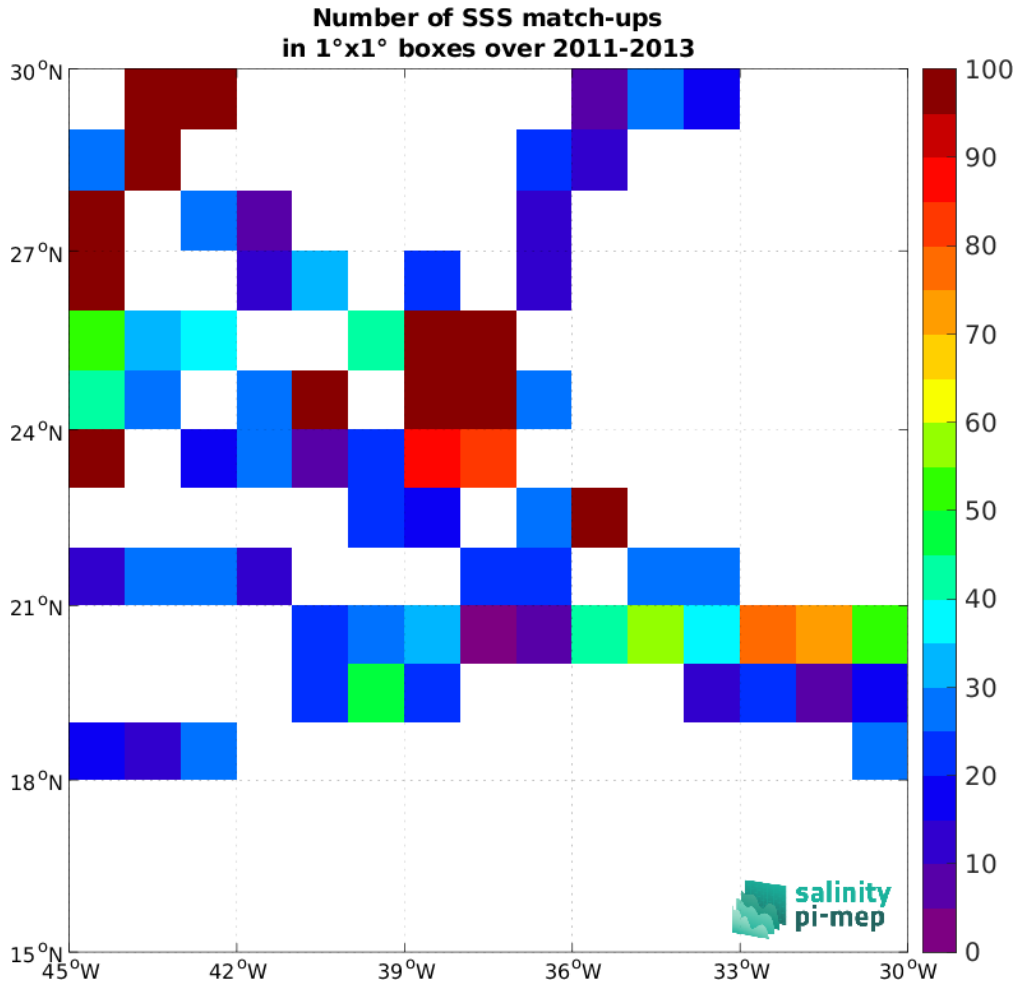
Figure 5: Number of SSS match-ups between TSG (SAMOS) SSS and the Aquarius SSS L3 CAP v5 - 7-Day running (JPL) SSS product for the SPURS 1 Pi-MEP region over 1^\circ \times 1^\circ boxes and for the full satellite product period.
