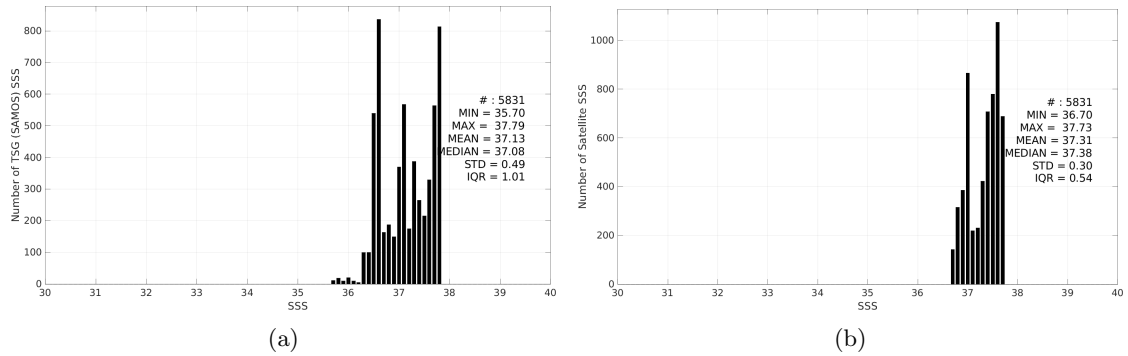
Figure 3: Histograms of SSS from TSG (SAMOS) (a) and Aquarius SSS L3 CAP v5 - 7-Day running (JPL) (b) considering all match-up pairs per bins of 0.1 over the SPURS 1 Pi-MEP region and for the full satellite product period.
