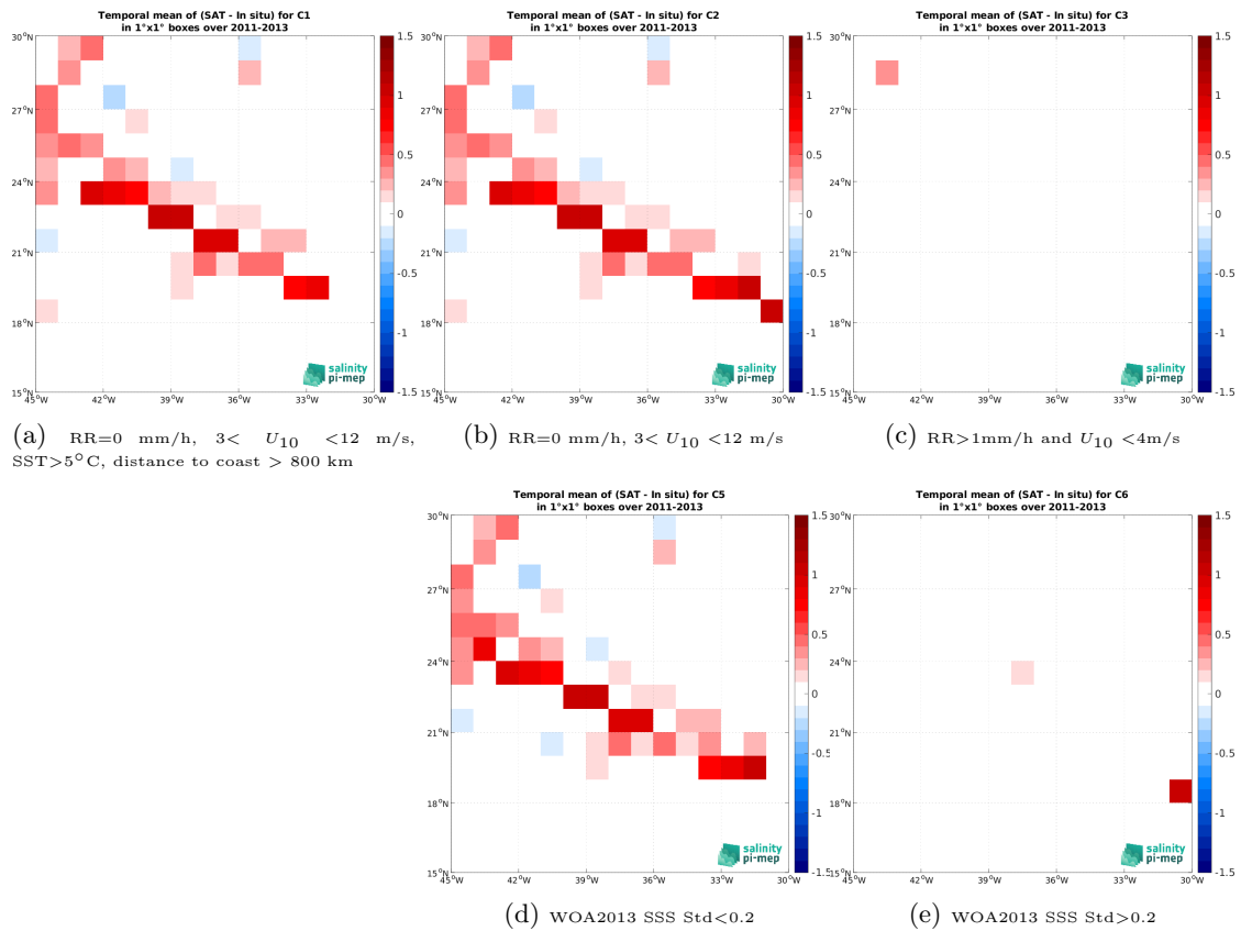
Figure 14: Temporal mean gridded over spatial boxes of size 1^\circ \times 1^\circ of \Delta SSS (Aquarius SSS L3 CAP v5 - 7-Day running (JPL) - TSG (SAMOS)) for 5 different subdatasets corresponding to:RR=0 mm/h, 3 < U_{10} < 12 m/s, SST>5°C, distance to coast > 800 km (a), RR=0 mm/h, 3 < U_{10} < 12 m/s (b), RR>1mm/h and U_{10} < 4 m/s (c), WOA2013 SSS Std<0.2 (d), WOA2013 SSS Std>0.2 (e).
