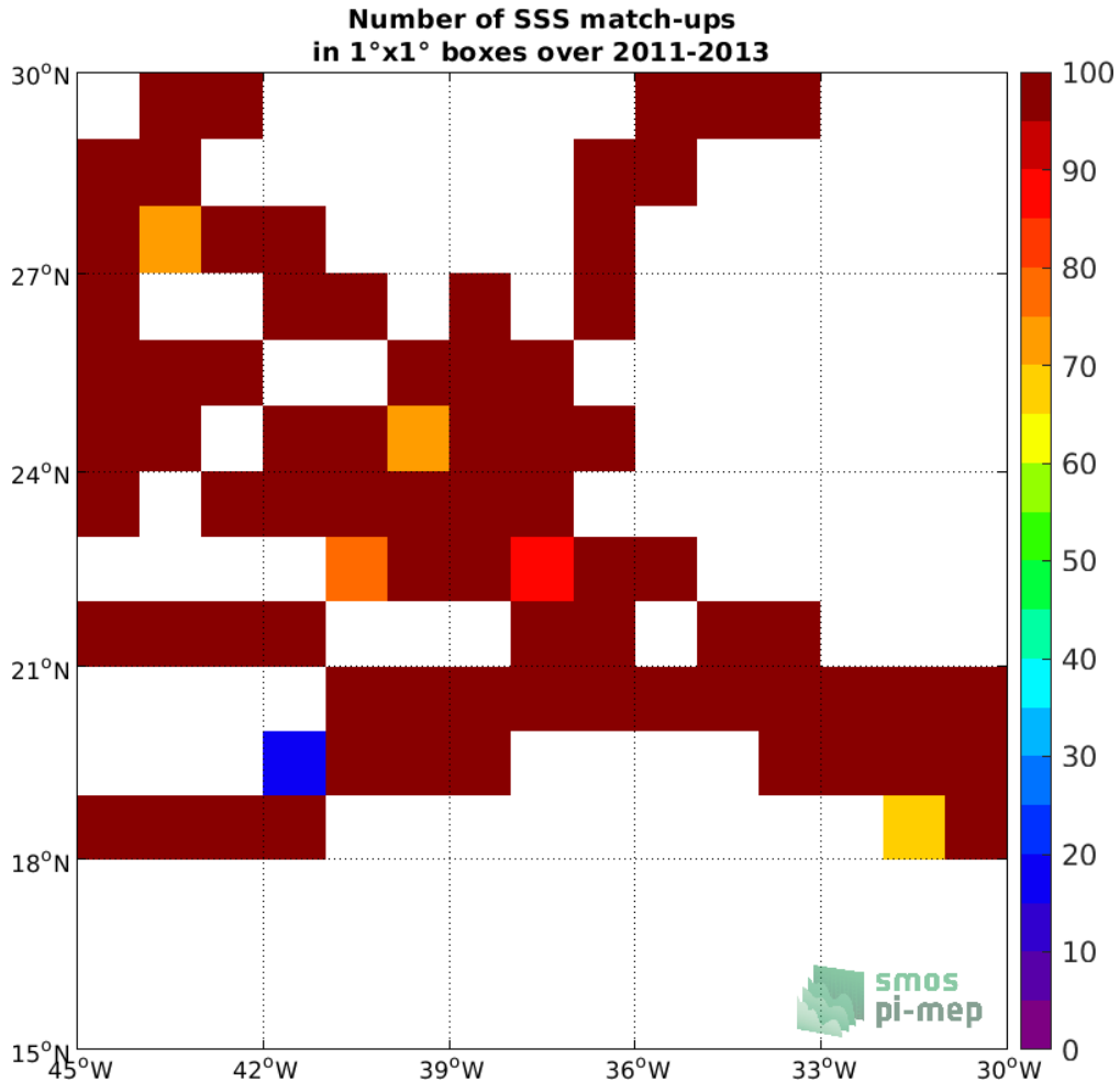
Figure 4: Number of SSS match-ups between TSG (SAMOS) SSS and the Aquarius SSS L3 CAP v5 - 7-Day running (JPL) SSS product for the SPURS 1 Pi-MEP region over 1°x1° boxes and for the full satellite product period.
