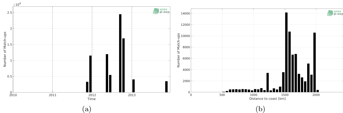
Figure 1: Number of match-ups between TSG (SAMOS) and Aquarius SSS L3 CAP v5 - 7-Day running (JPL) SSS as a function of time (a) and as function of the distance to coast (b) over the SPURS 1 Pi-MEP region and for the full satellite product period.
